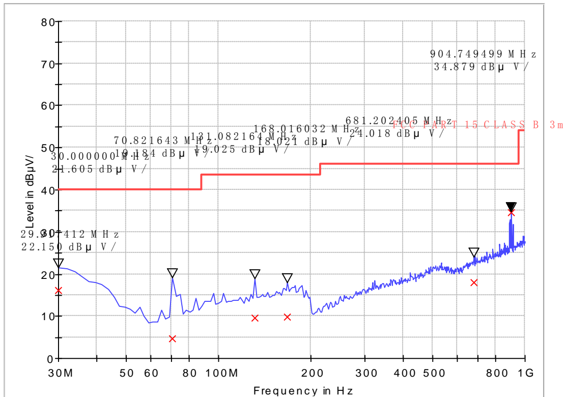
EMI Sweep-3M(30-1G)
