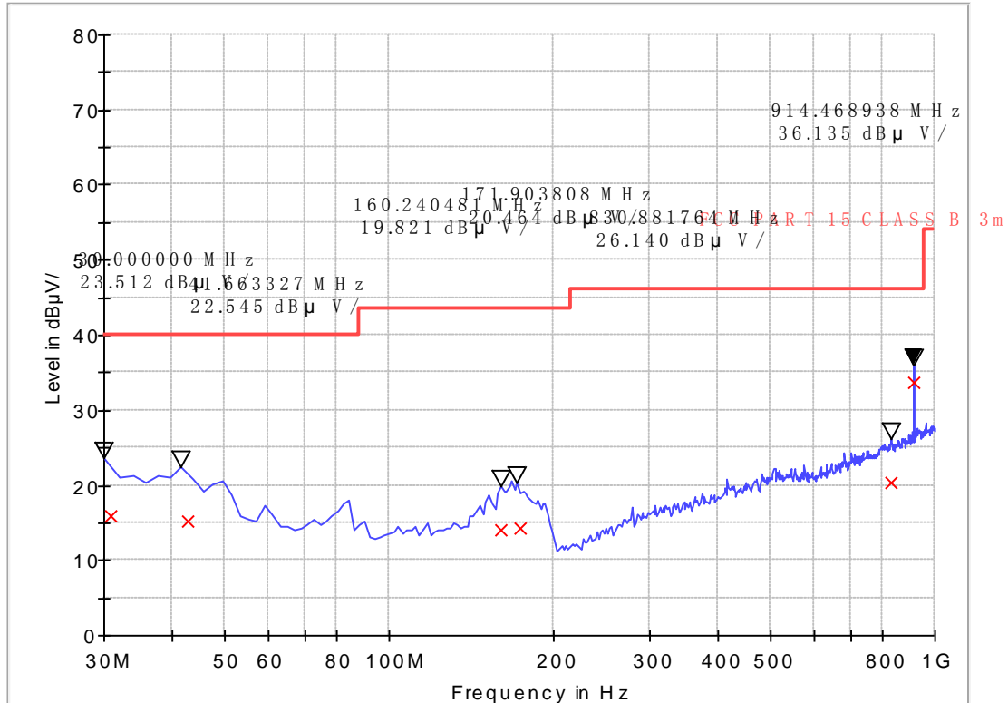
EMI Sweep-3M(30-1G)
