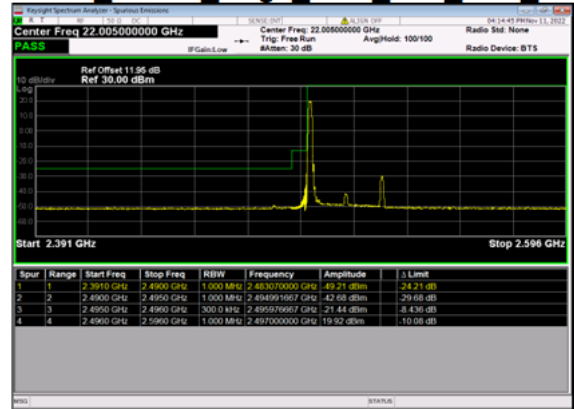
n41(30M)_DFT-s-OFDM QPSK Edge 1RB Left Low CH
