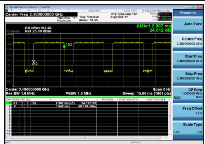
8DPSK,2480,3DH5,Transmission Time
