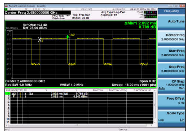
DQPSK,2480,2DH5,Transmission Time
