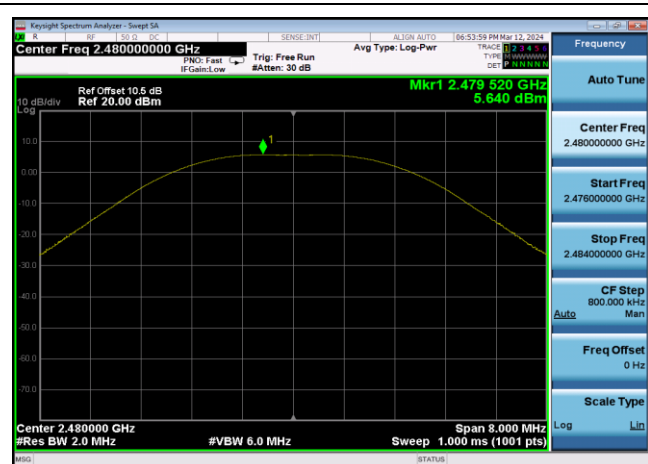
Output Power: 2480MHz – 2Mbps
