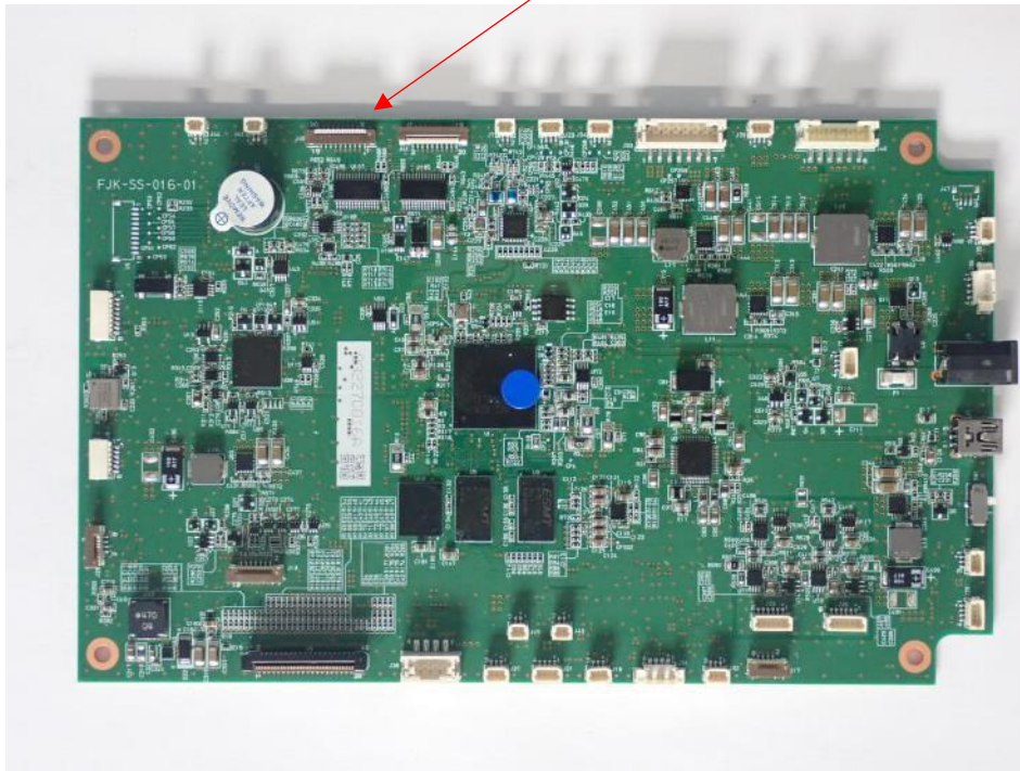
Mainboard (Front)
