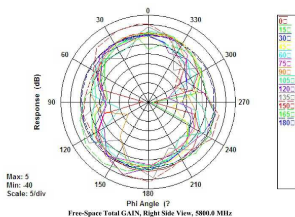
Free-Space Total GAIN, Right Side View, 5800.0 MHz
