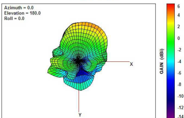
Free-Space Total GAIN, Bottom View, 5800.0 MHz
