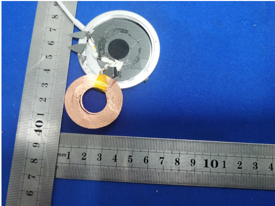
Antenna photo
