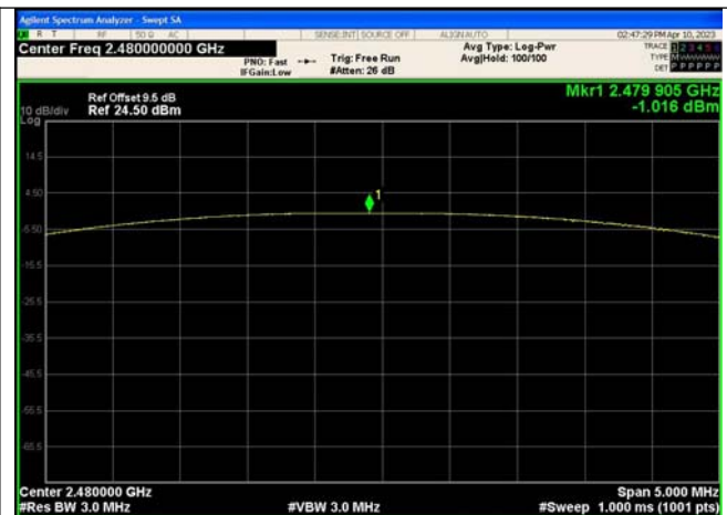
Peak Output Power \pi/4 DQPSK_Channel 78
