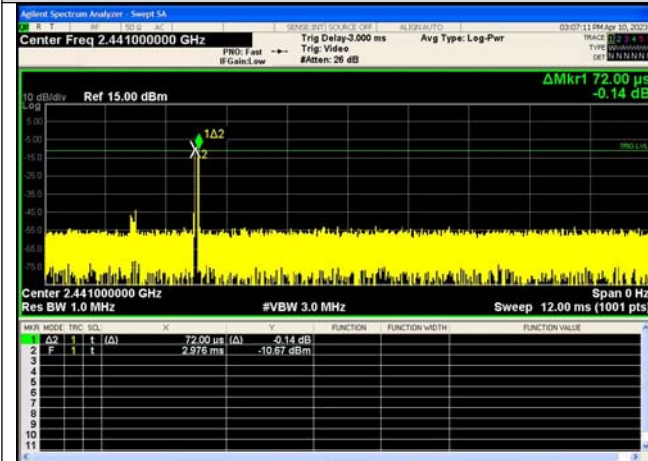
Pulse Width π/4DQPSK_2-DH3
