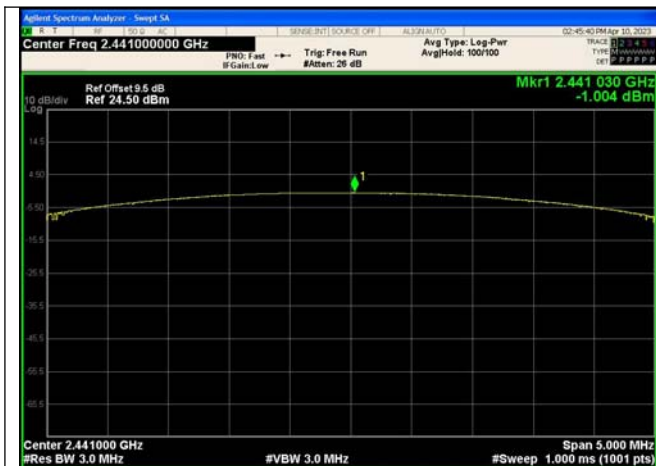
Peak Output Power \pi/4 DQPSK_Channel 39
