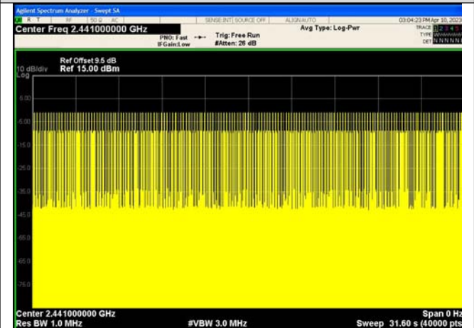
Number of Pulses in 31.6 seconds π/4DQPSK_2-DH1
