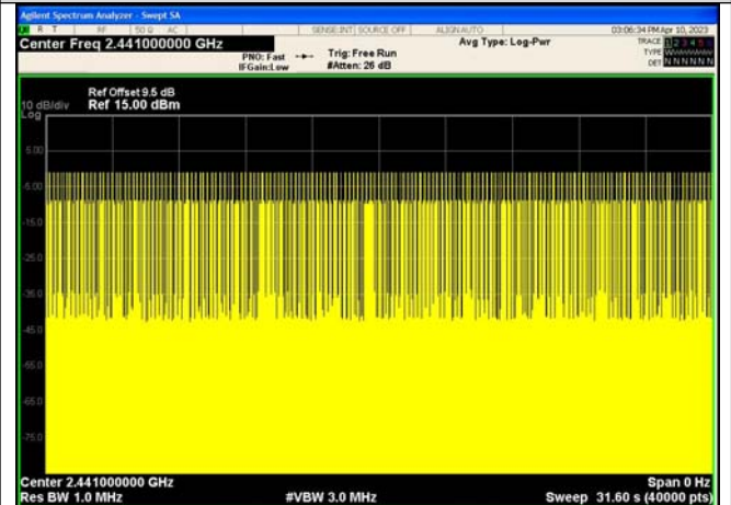
Number of Pulses in 31.6 seconds π/4DQPSK_2-DH3
