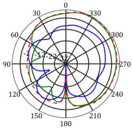
frequency=2450MHz, X-Z Plane
