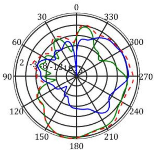
frequency=5150MHz, X-Y Plane
