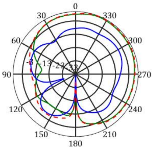
frequency=2500MHz, X-Z Plane
