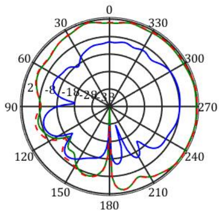
frequency=5500MHz, X-Z Plane
