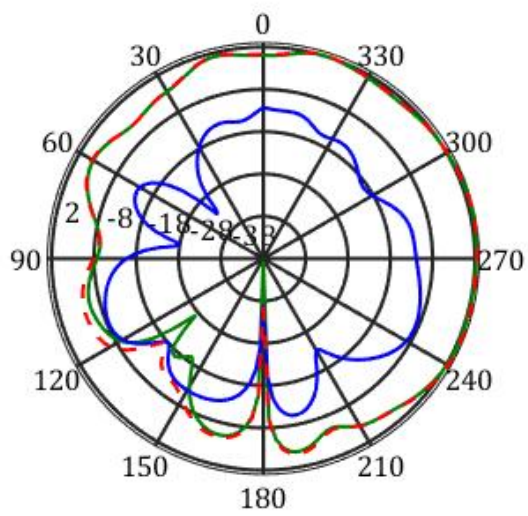
frequency=5150MHz, Y-Z Plane
