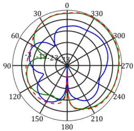
frequency=2400MHz, X-Z Plane
