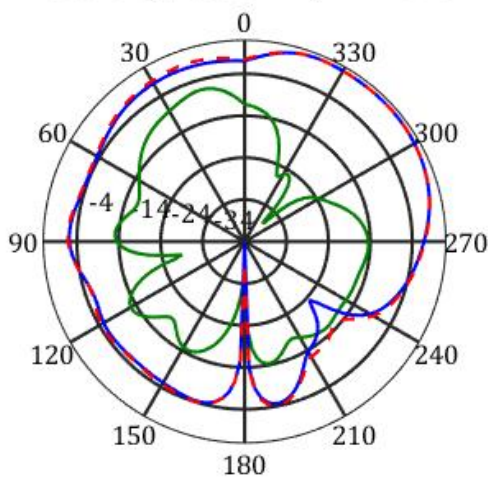
frequency=5850MHz, Y-Z Plane
