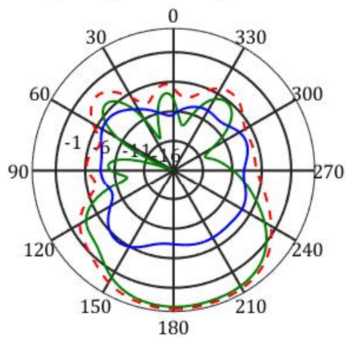
frequency=2400MHz, X-Y Plane
