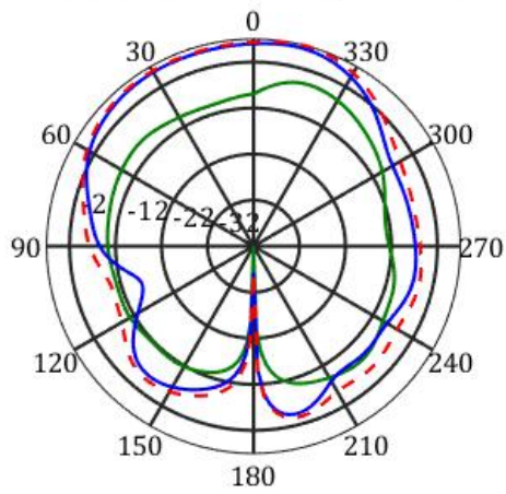
frequency=2450MHz, Y-Z Plane
