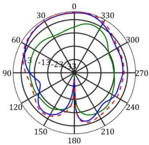
frequency=2500MHz, Y-Z Plane
