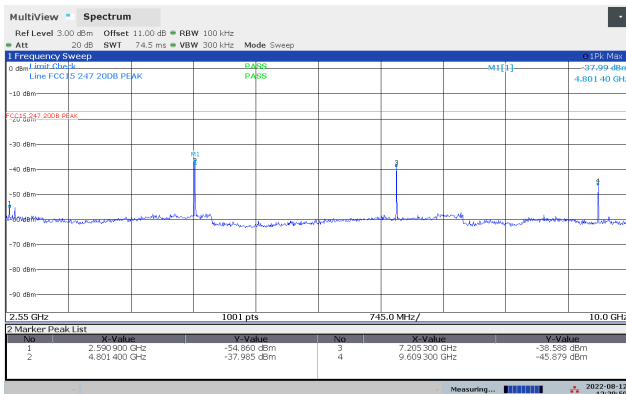
Conducted Emissions 2.55-10 GHz, 2402 MHz, 2Mb
