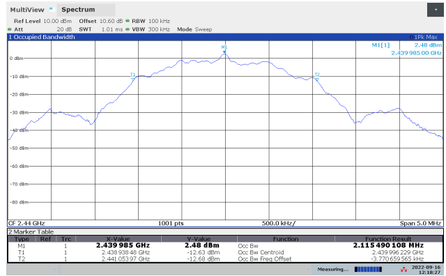
99% Occupied BW, 2Mb
