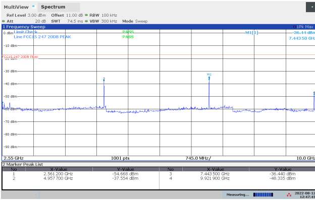
Conducted Emissions 2.55-10 GHz, 2480 MHz, 2Mb
