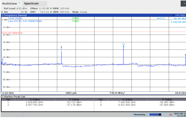
Conducted Emissions 2.55-10 GHz, 2480 MHz, 1Mb
