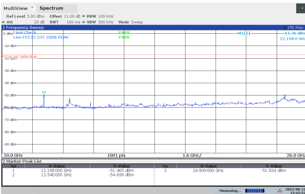
Conducted Emissions 10-26 GHz, 2480 MHz, 1Mb
