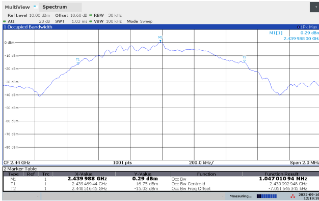
99% Occupied BW, 1Mb
