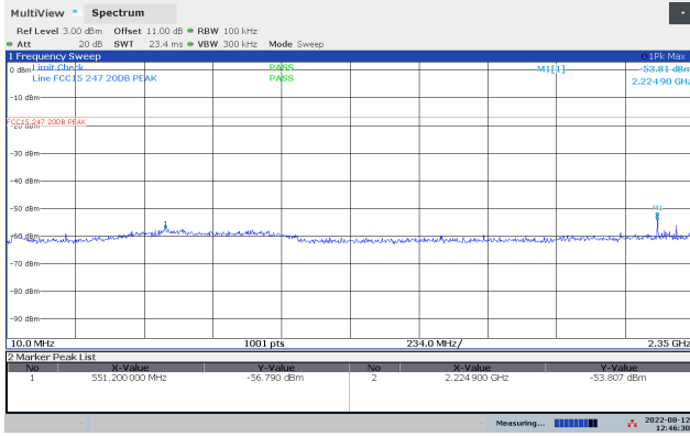
Conducted Emissions 10-2350 MHz, 2480 MHz, 2Mb
