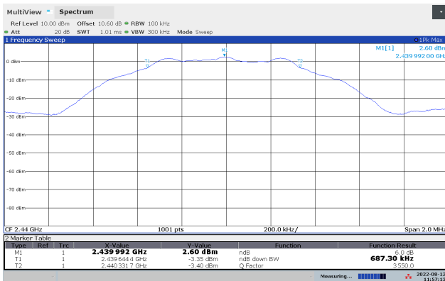
DTS BW, 2440 MHz, 1Mb
