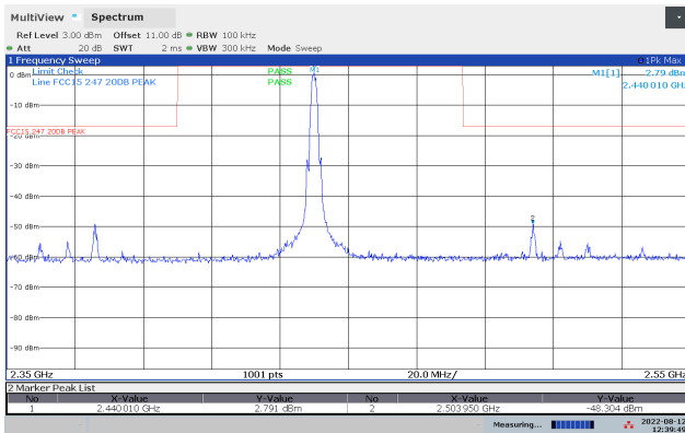
Conducted Emissions 2350-2550 MHz, 2440 MHz, 2Mb
