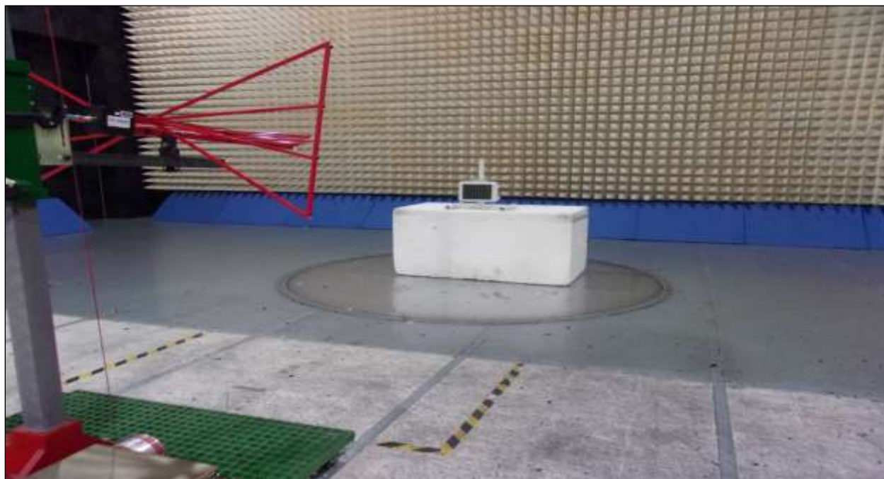
Figure 1: Radiated Emissions, 30MHz – 1GHz
