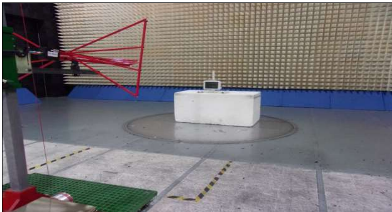
Figure 3: FCC 15.247 RSE, 30MHz – 1GHz
