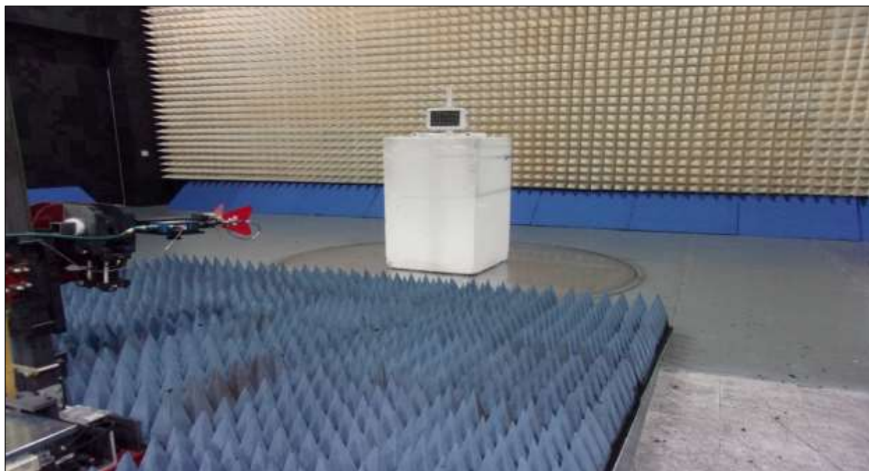
Figure 3: FCC 15.247 RSE, 1GHz – 18GHz
