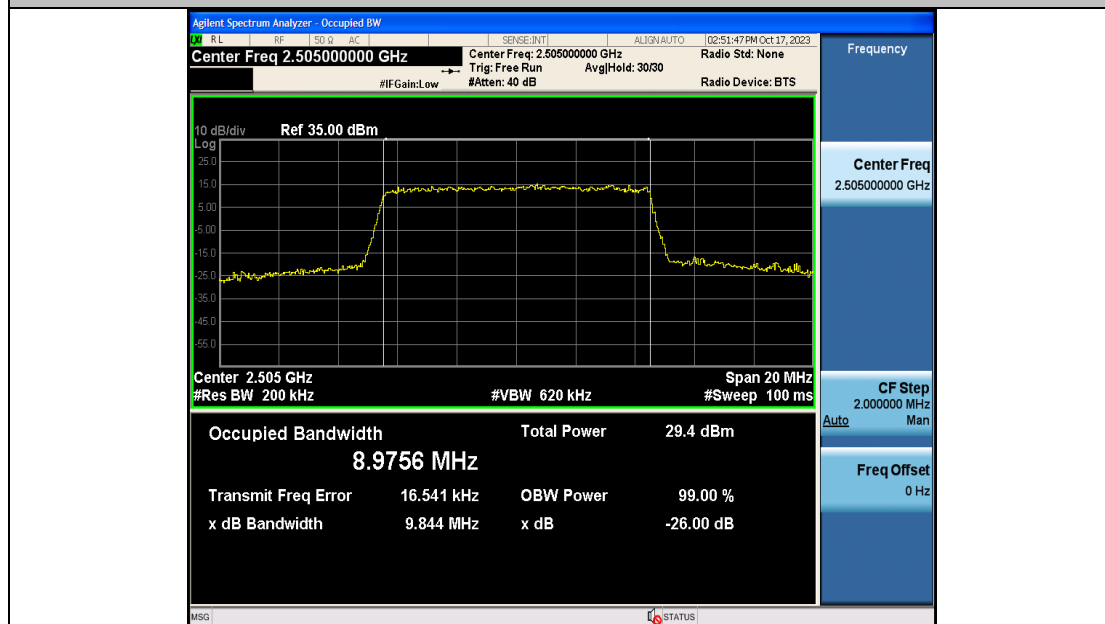
Band7-10MHz-16QAM-20800-50RB#0-PASS
