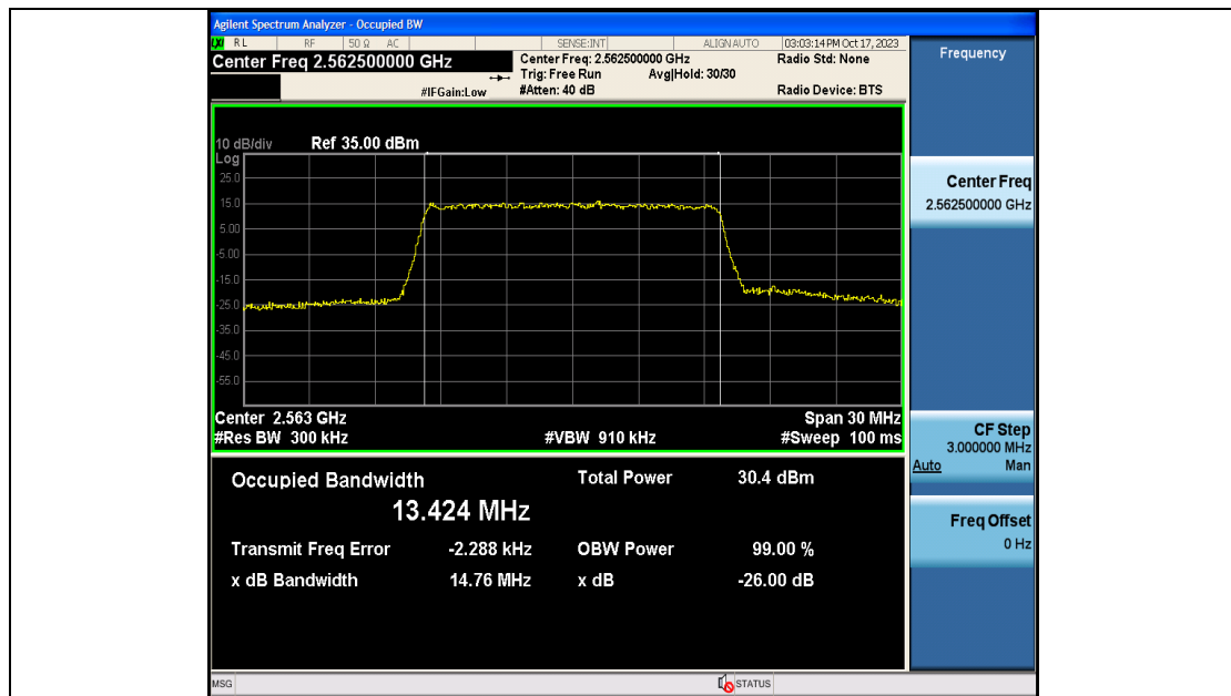
Band7-15MHz-QPSK-21375-75RB#0-PASS
