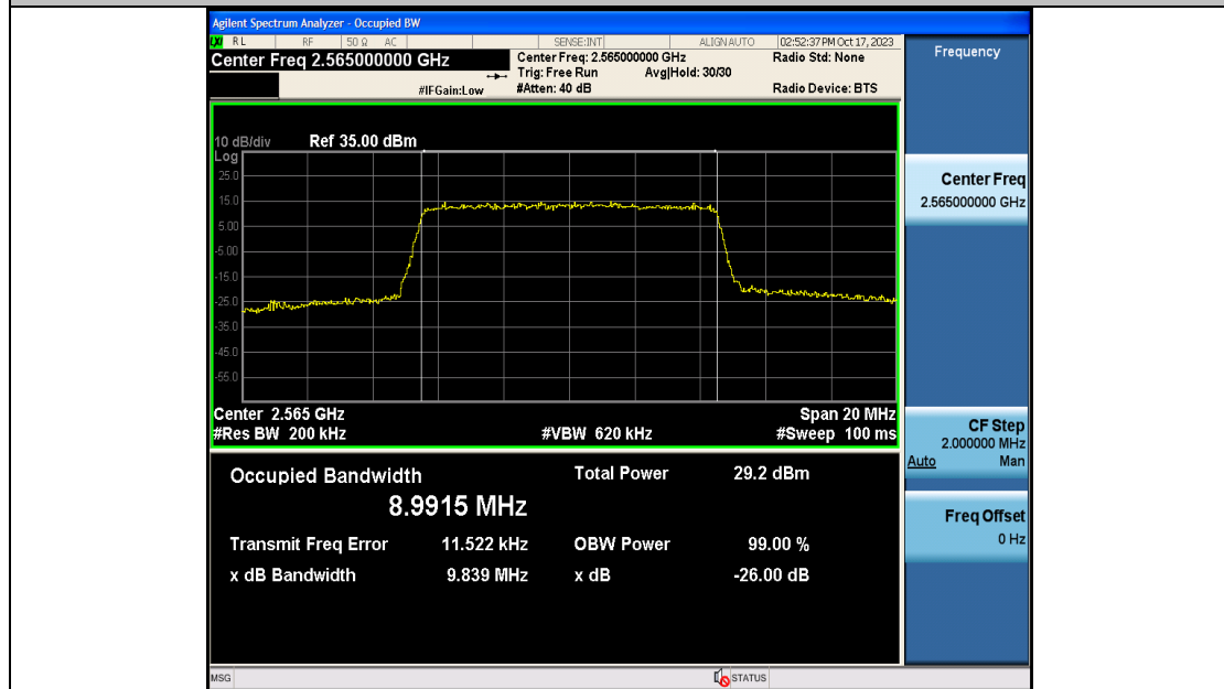
Band7-10MHz-16QAM-21400-50RB#0-PASS
