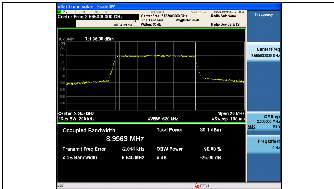
Band7-10MHz-QPSK-21400-50RB#0-PASS
