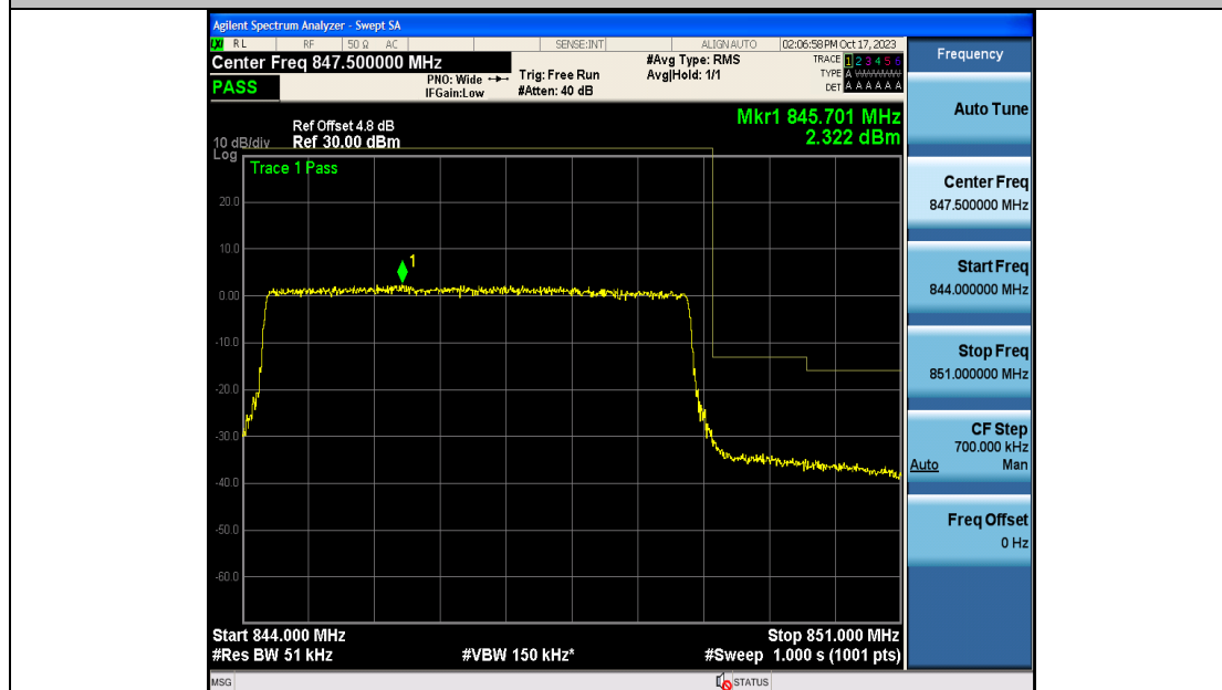
Band5_5MHz_QPSK_20625_25RB#0
