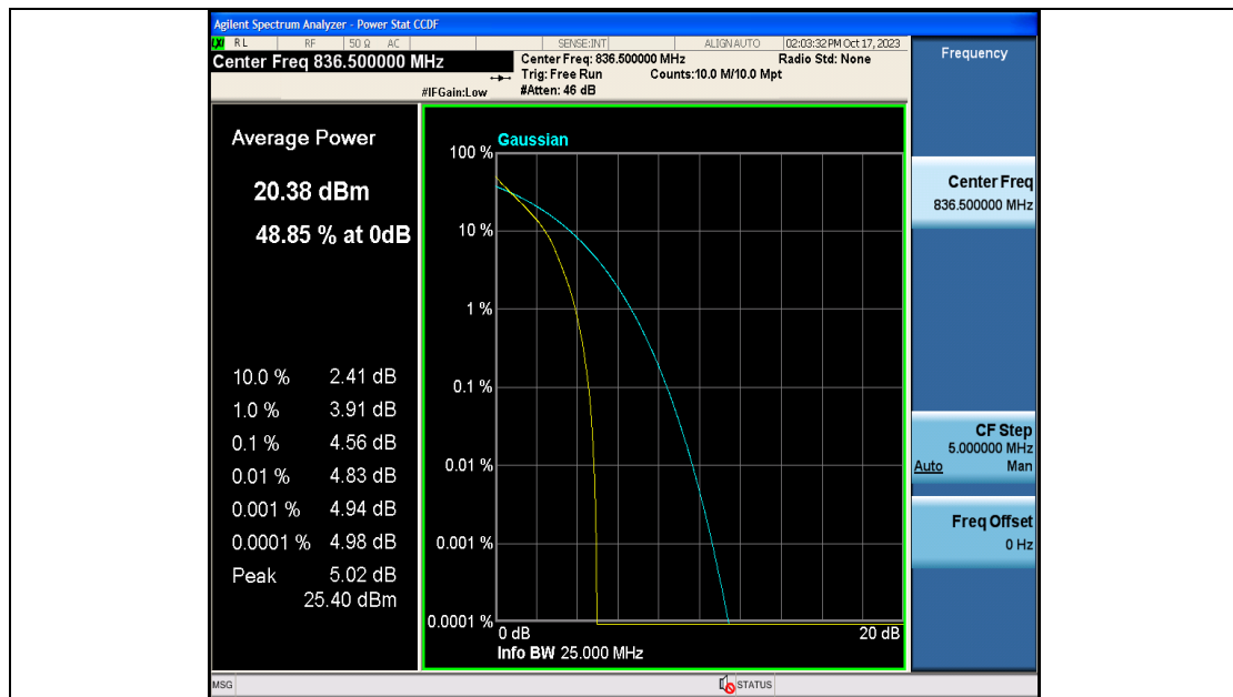
Band5-3MHz-QPSK-20525-15RB#0-PASS
