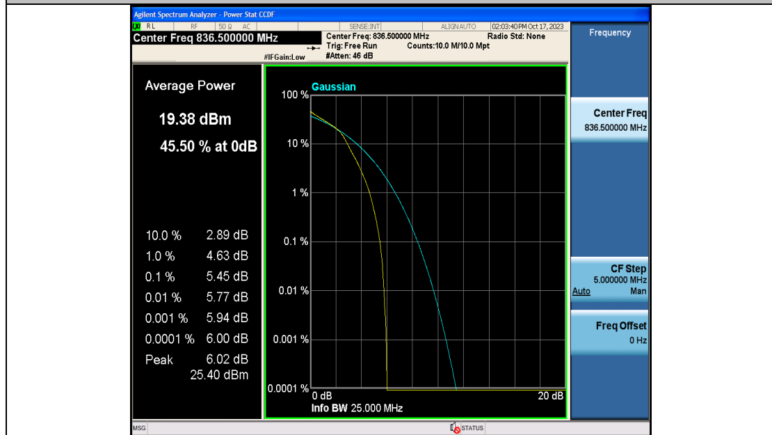
Band5-3MHz-16QAM-20525-15RB#0-PASS
