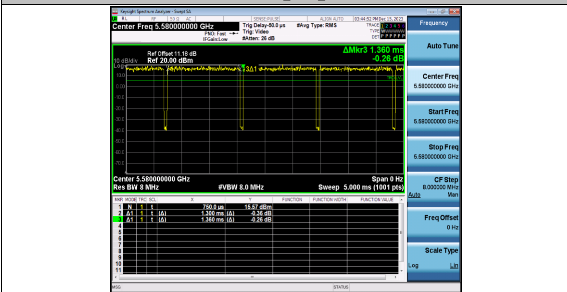
11N20SISO_Ant 0_5580
