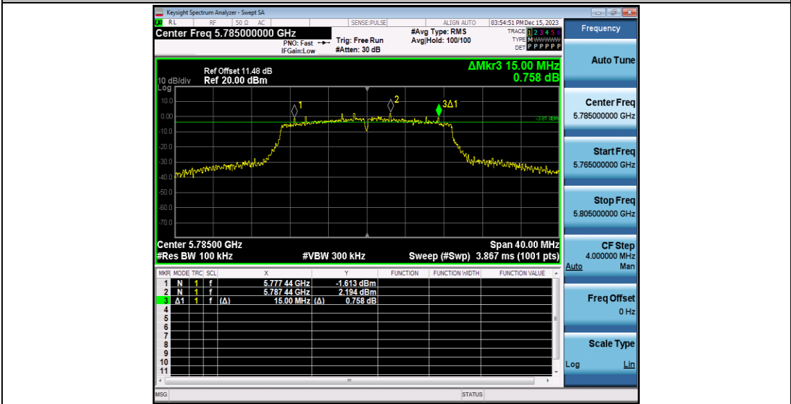
11N20SISO_Ant 0_5785
