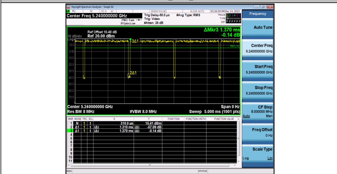
11N20SISO_Ant 0_5240
