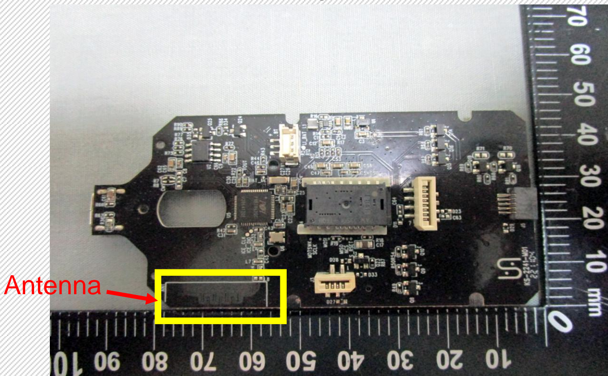
< PCB-F >
