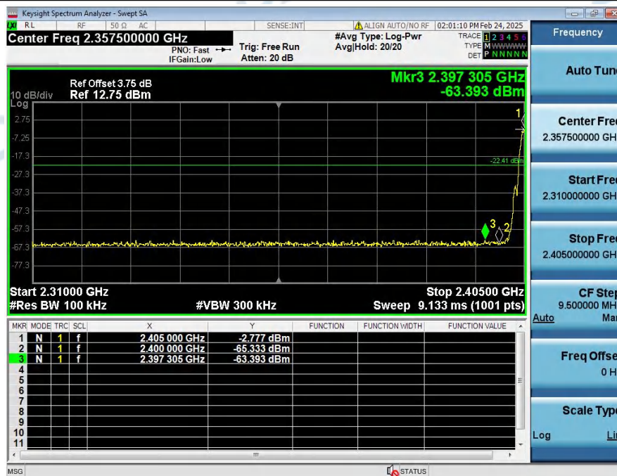
2_Bandedge_NVNT_ANT1_1Mbps_2405
