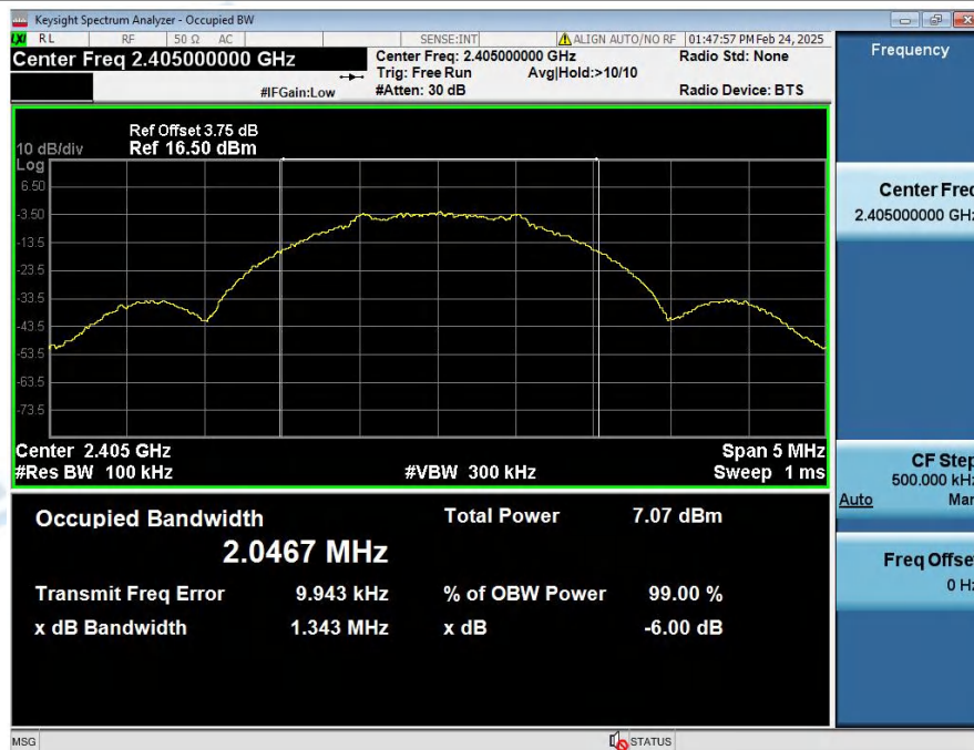
-6dB_Bandwidth_NVNT_ANT1_1Mbps_2405
