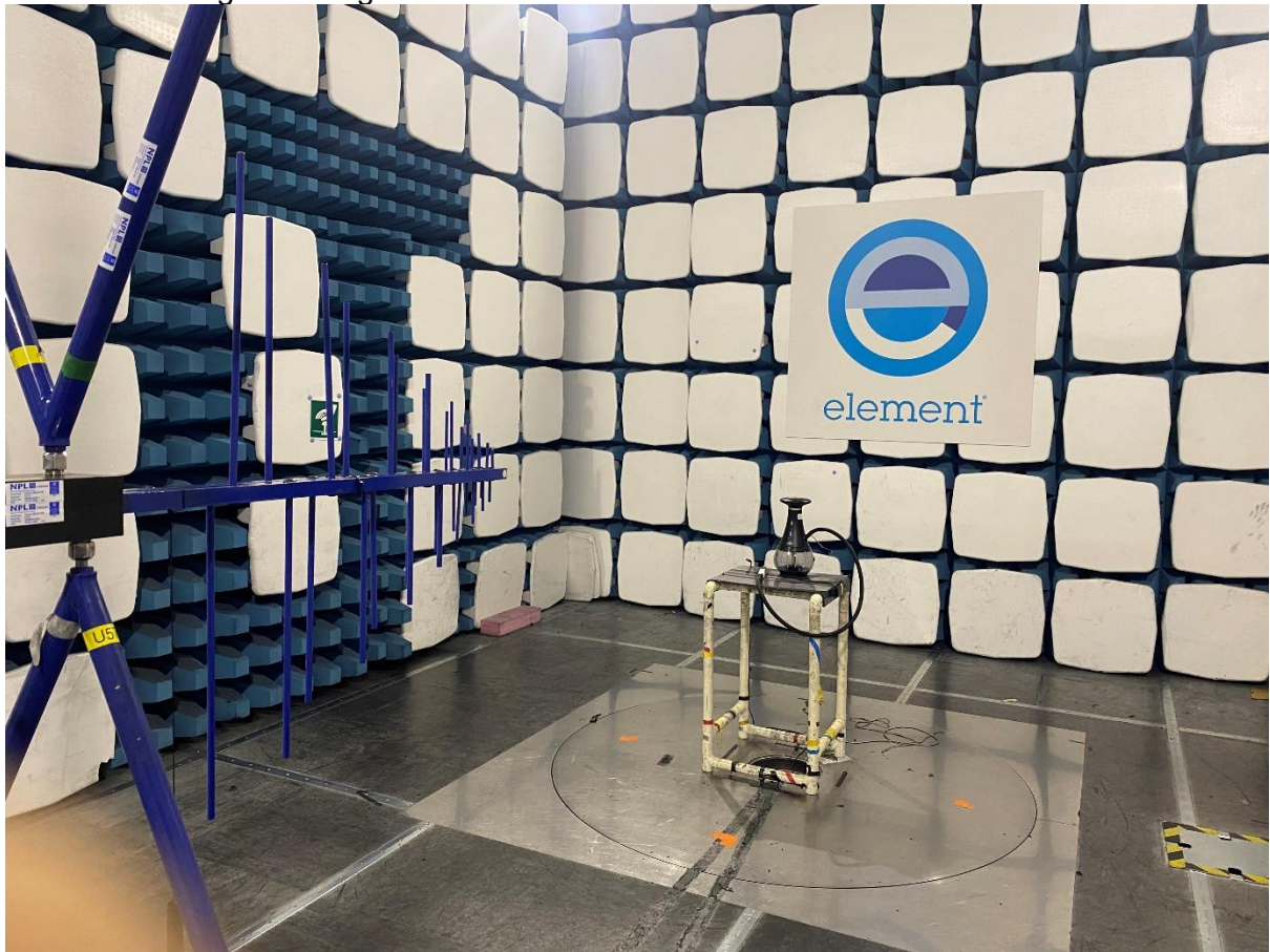
Radiated Testing with Bilog Antenna
