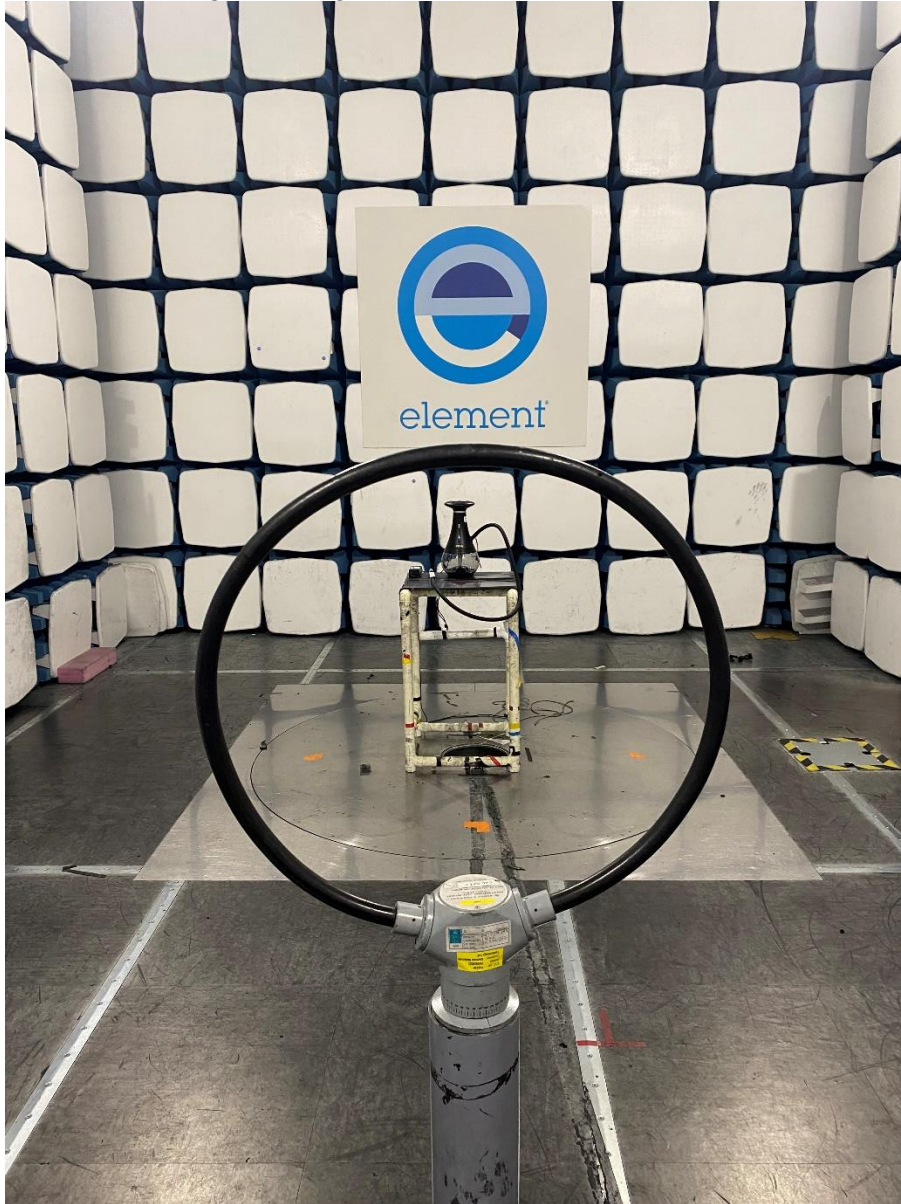
Radiated Testing with Magnetic Loop antenna
