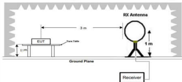
Figure 1. Below 30MHz
