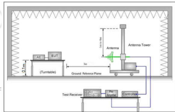
Figure 2. 30MHz-1GHz
