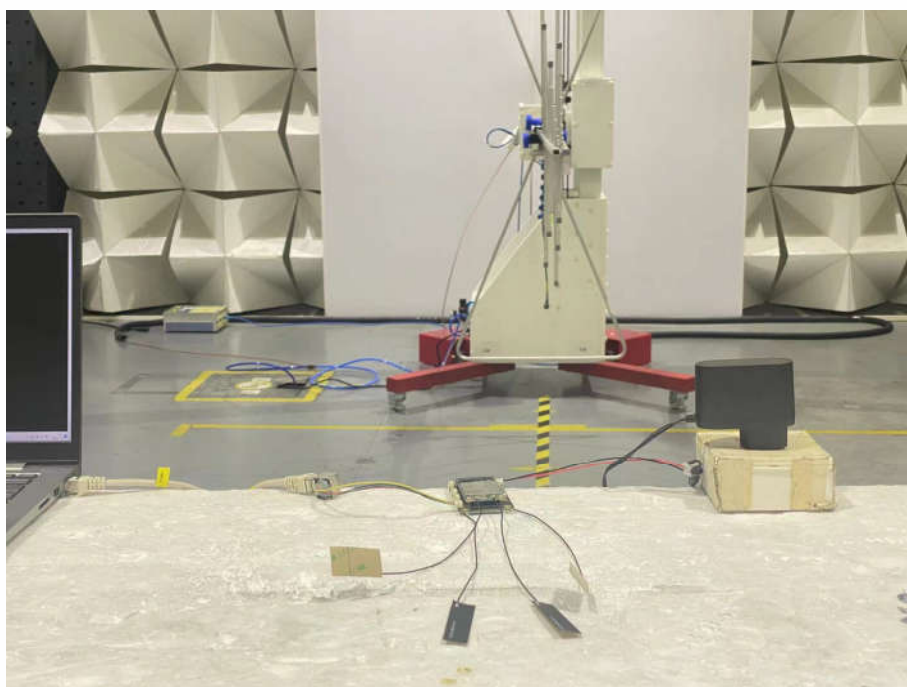
Radiated spurious emission Test Setup-2(close up)(Below 1GHz)
