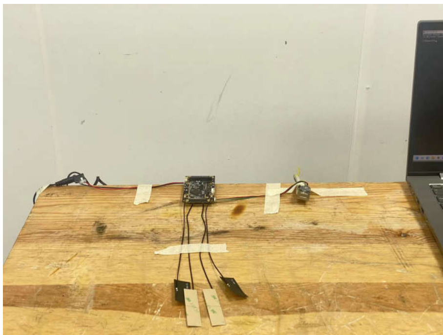
Conducted Emissions Test Setup-2(close up)
