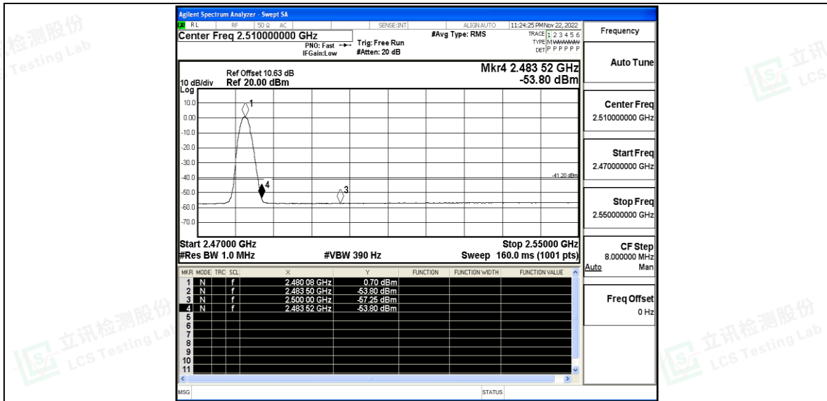
2DH5_Ant_High_2480_Peak
