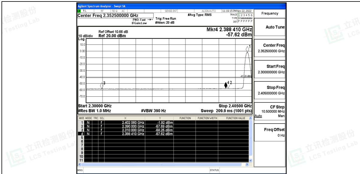
2DH5_Ant_Low_2402_Peak
