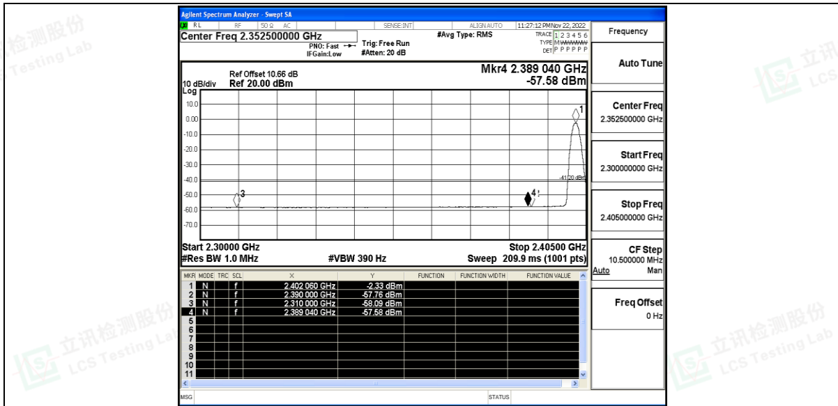
3DH5_Ant_Low_2402_Peak
