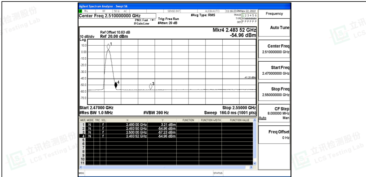
DH5_Ant_High_2480_Peak
