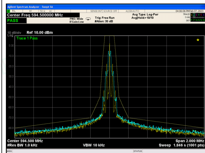
Channel 15 / 594.5 MHz
