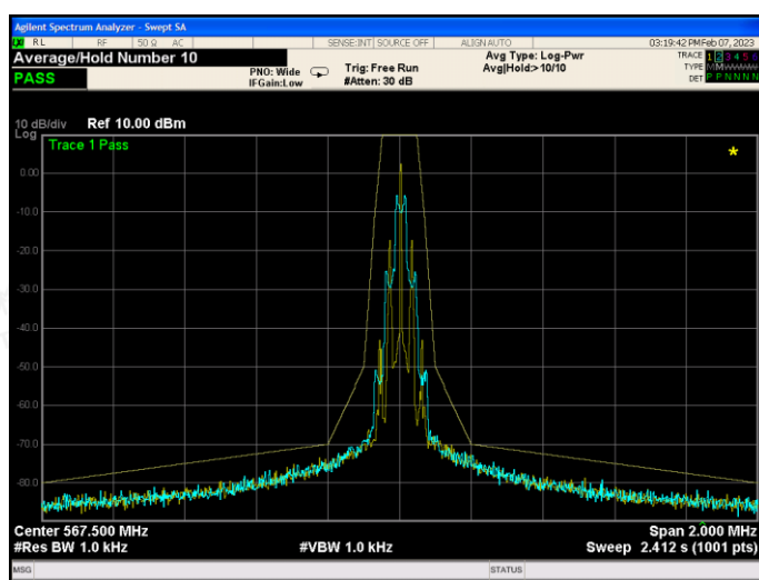
Channel 8 / 567.5 MHz
