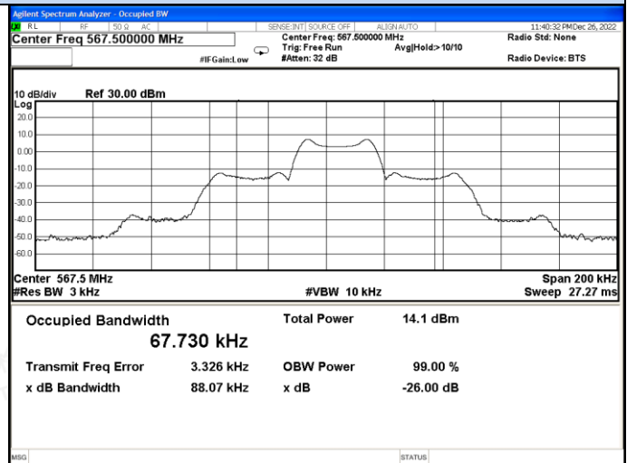
Channel 8 / 567.5 MHz
