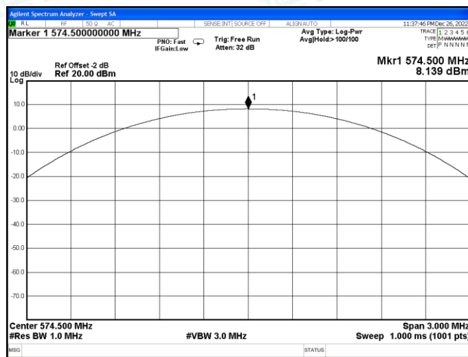
Channel 3 / 574.5 MHz
