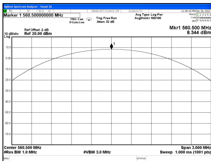
Channel 1 / 560.5 MHz
