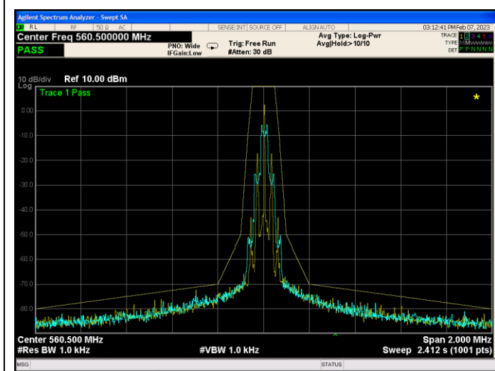
Channel 1 / 560.5 MHz
