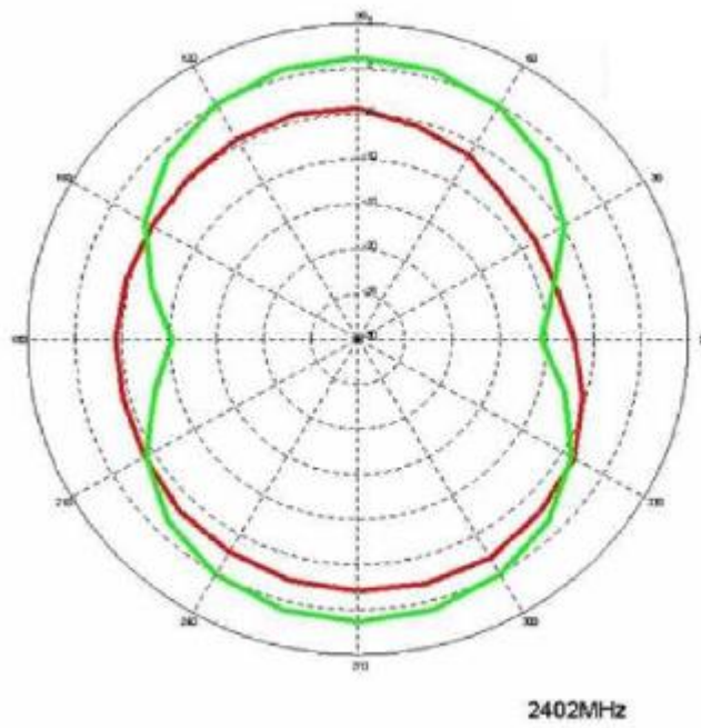
Radiation pattern @2.402GHz
