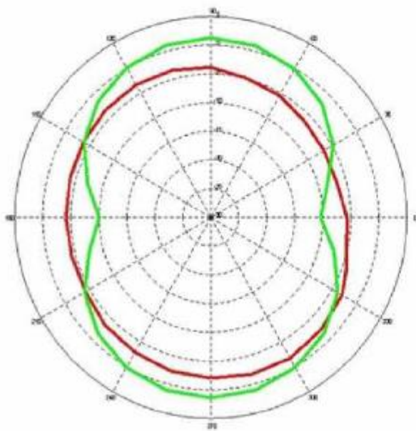
Radiation pattern @2.441GHz
