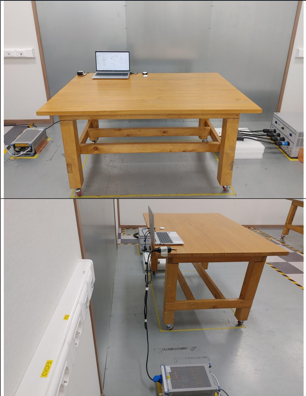
Photo of test set up for conducted voltage emissions Test configuration: Configuration 1 (Data transmitting)
