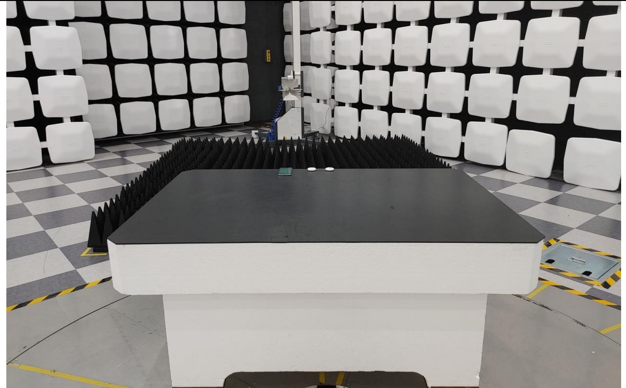
Photo of test set up for radiated emissions Test configuration: Configuration 2 (ECG measuring) [Above 1 GHz]
