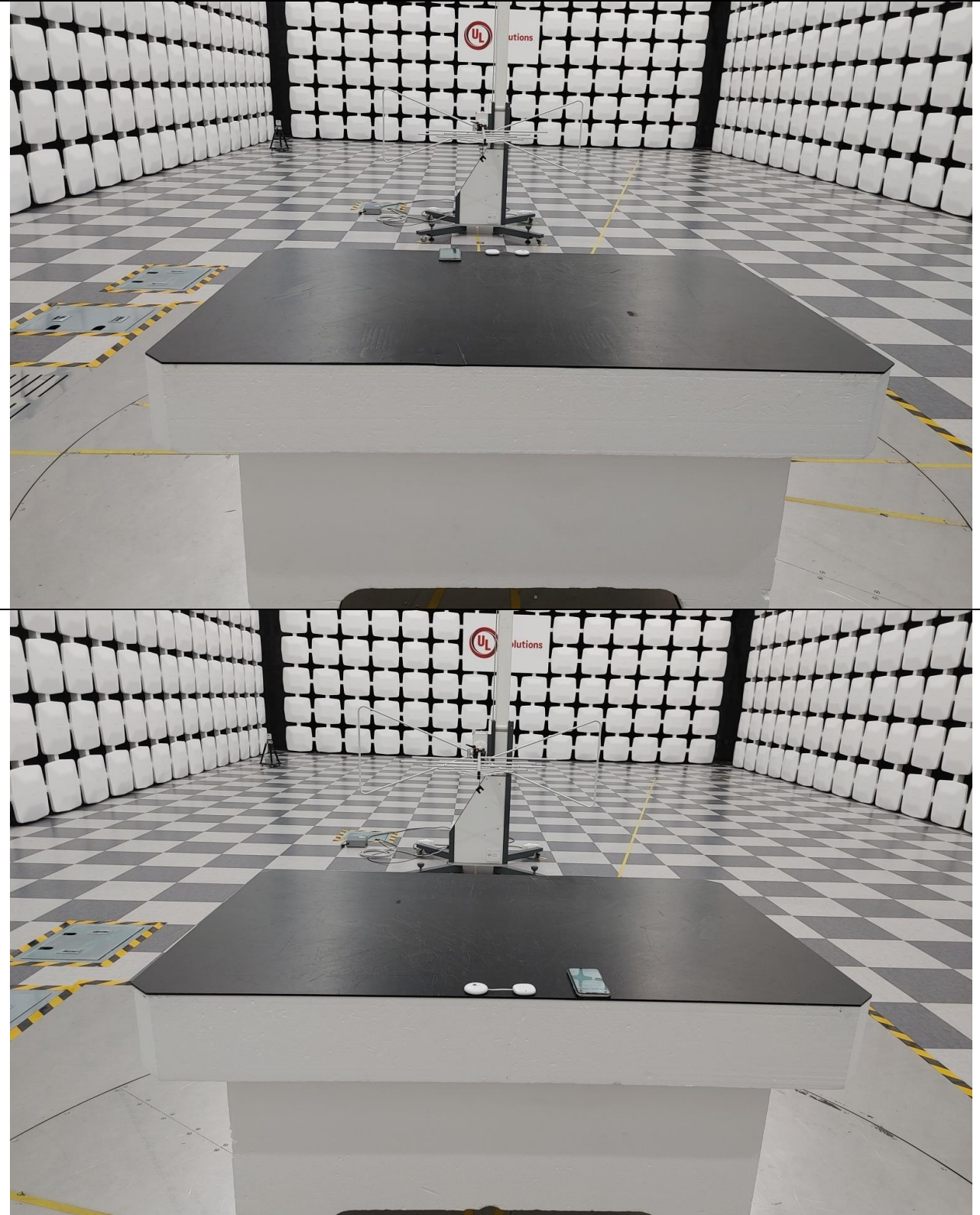
Photo of test set up for radiated emissions Test configuration: Configuration 2 (ECG measuring) [Below 1 GHz]
