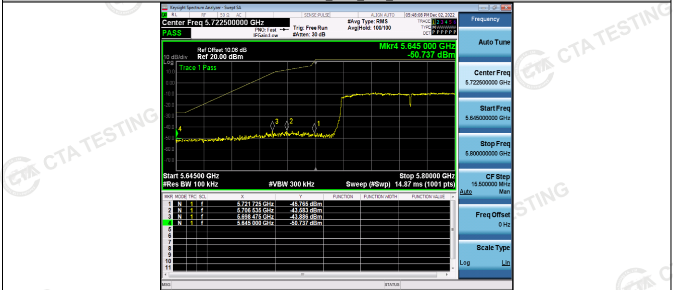
11AC80SISO_Ant1_High_5775
