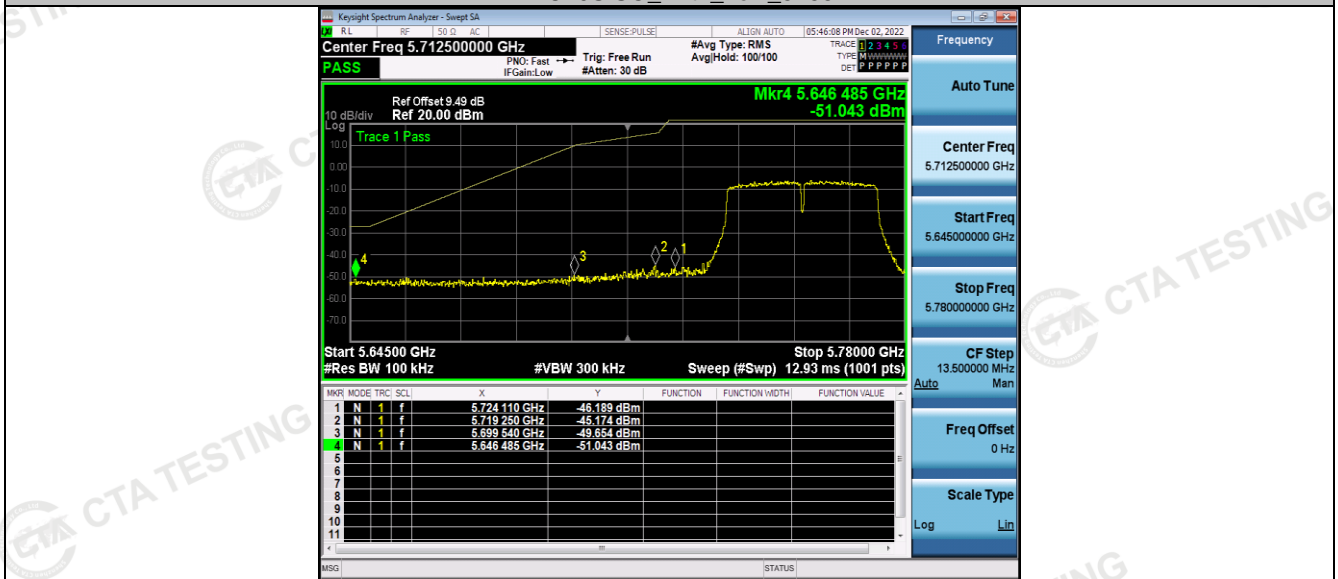
11AC40SISO_Ant1_High_5795
