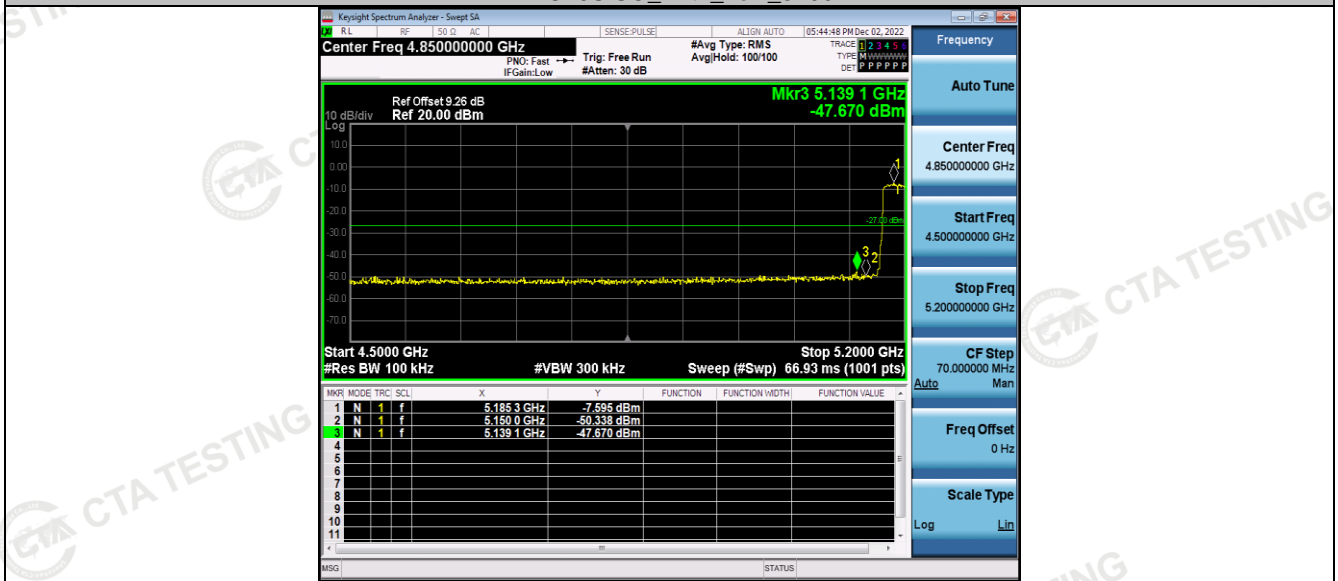
11AC40SISO_Ant1_High_5230
