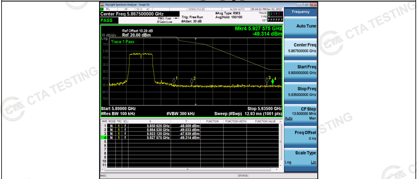
11AC40SISO_Ant1_Low_5755
