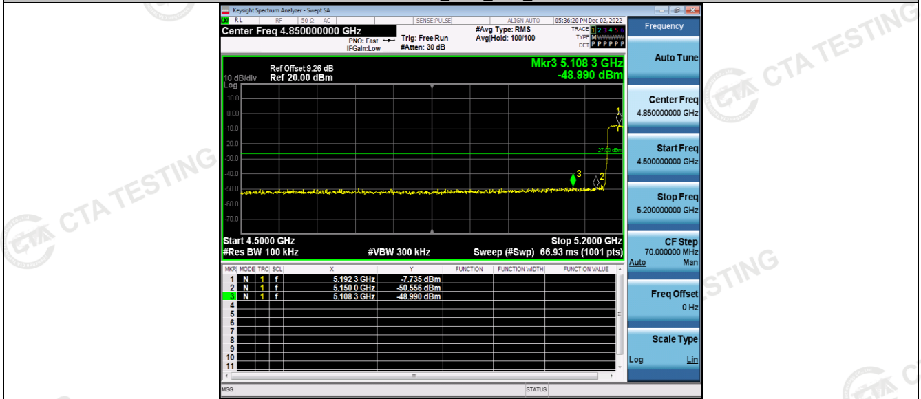
11N40SISO_Ant1_High_5230
