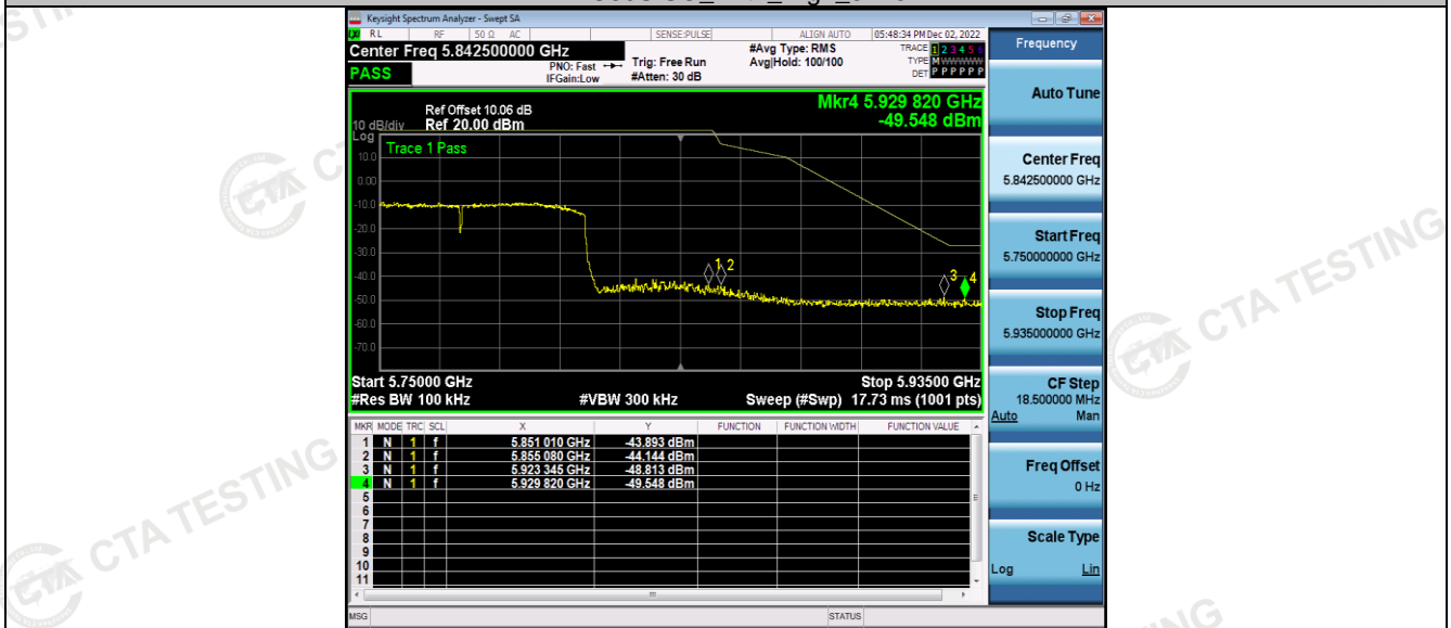
11AC80SISO_Ant1_High_5775
