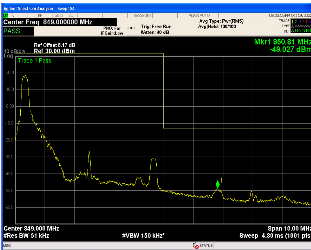
Band26b QPSK BW=5MHz Channel=27015 RB Size=1 Position=#Max
