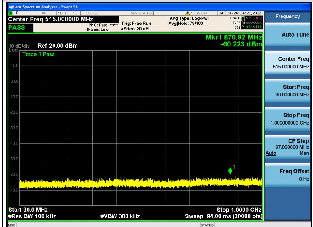
Test_Graph_802.11n40_ANT1_5795_MCS0_Frequency Band1
