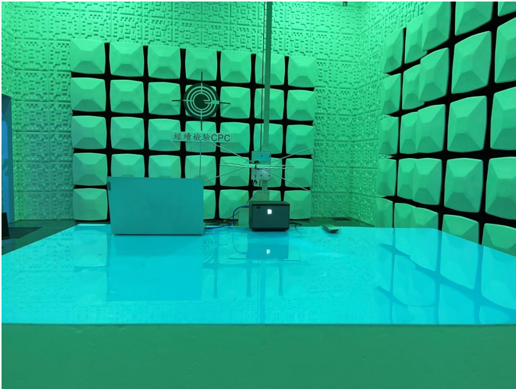
Setup Photo FCC ID: 2A9CO-LX5501
