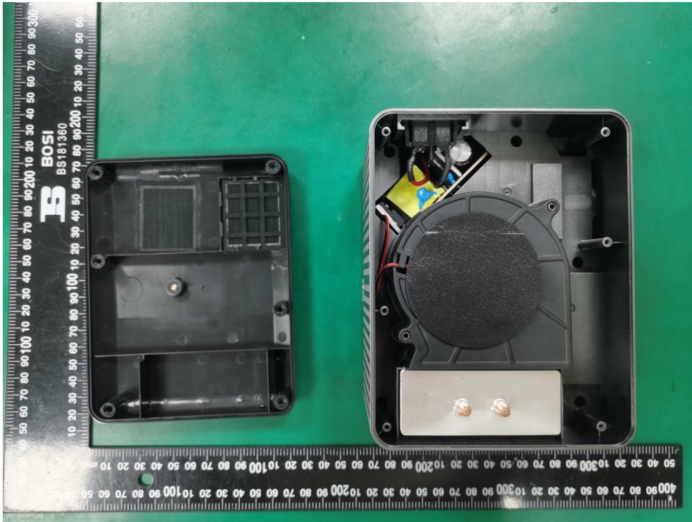
Internal Photo FCC ID: 2A9CO-LX5501
