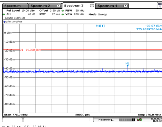
Left Side-WCDMA-Pre AGC
