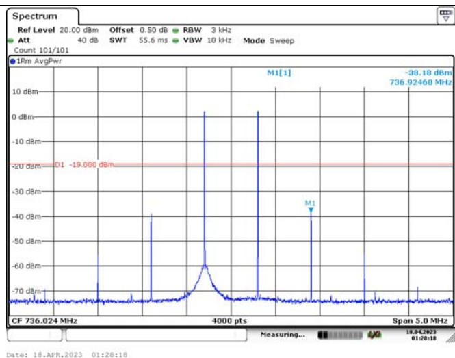
Upper 700MHz Band Downlink -Above AGC
