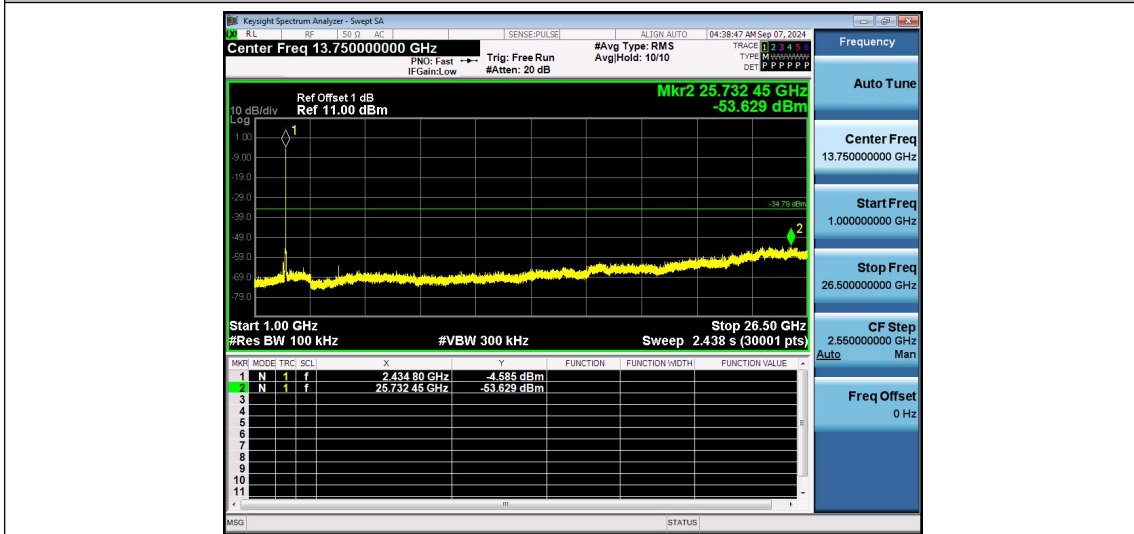
11G-Ant1-2437-1000~26500-PASS
