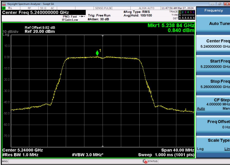
11A-Ant3-5240-PASS
