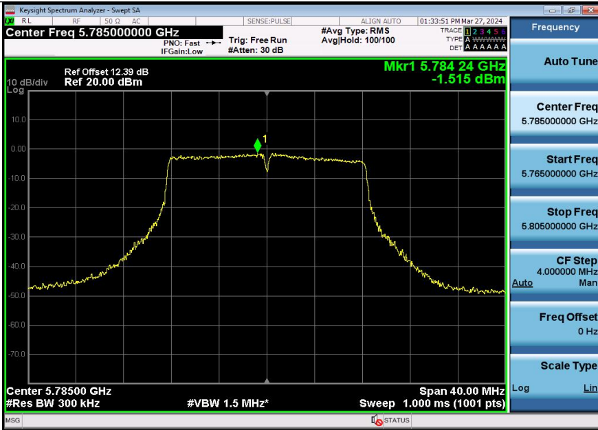
11A-Ant3-5785-PASS
