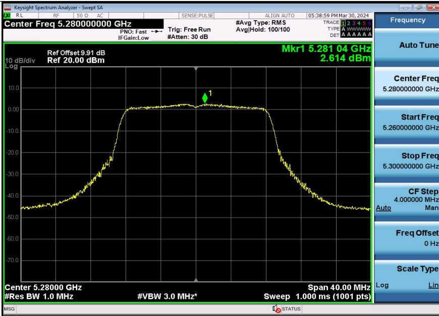
11A-Ant3-5280-PASS
