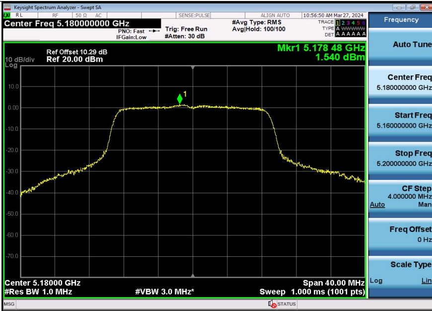
11AX20SISO-Ant2-5180-PASS
