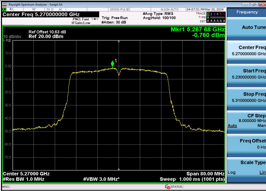
11AX40SISO-Ant2-5270-PASS
