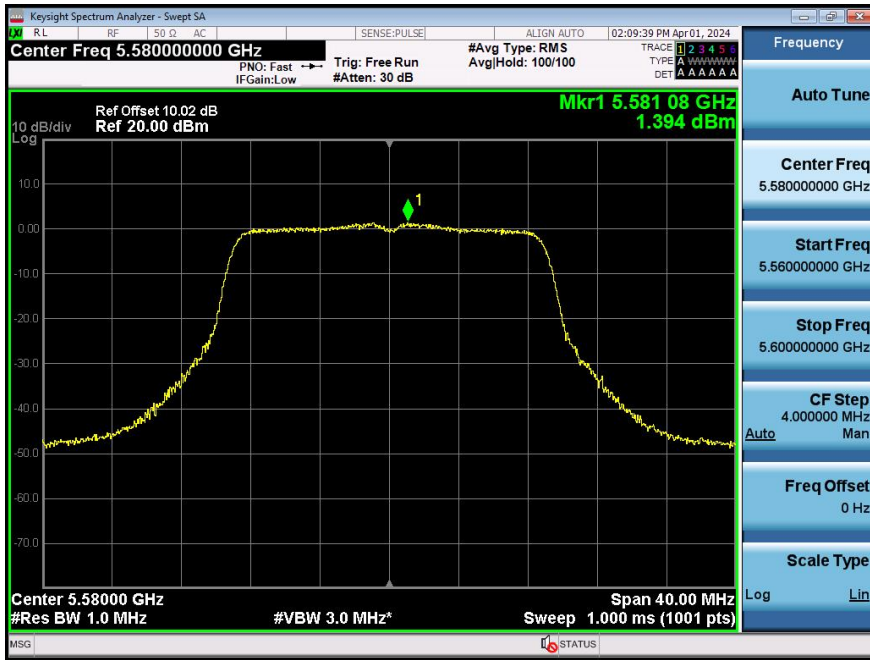
11AC20SISO-Ant2-5580-PASS
