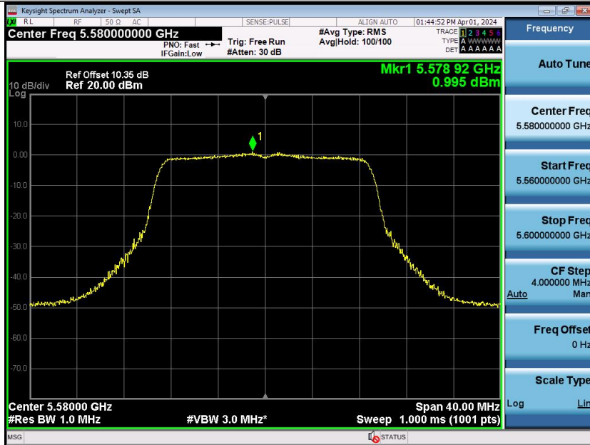
11N20SISO-Ant1-5580-PASS
