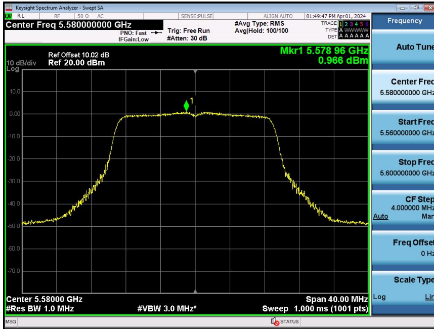
11AC20SISO-Ant1-5580-PASS
