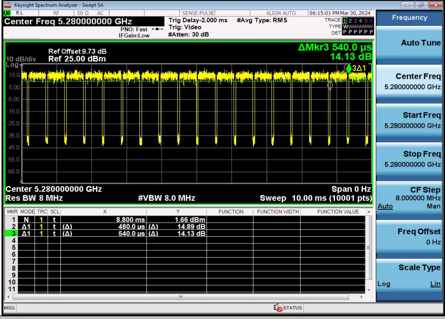
NTNV-11AX20SISO-Ant3-5280
