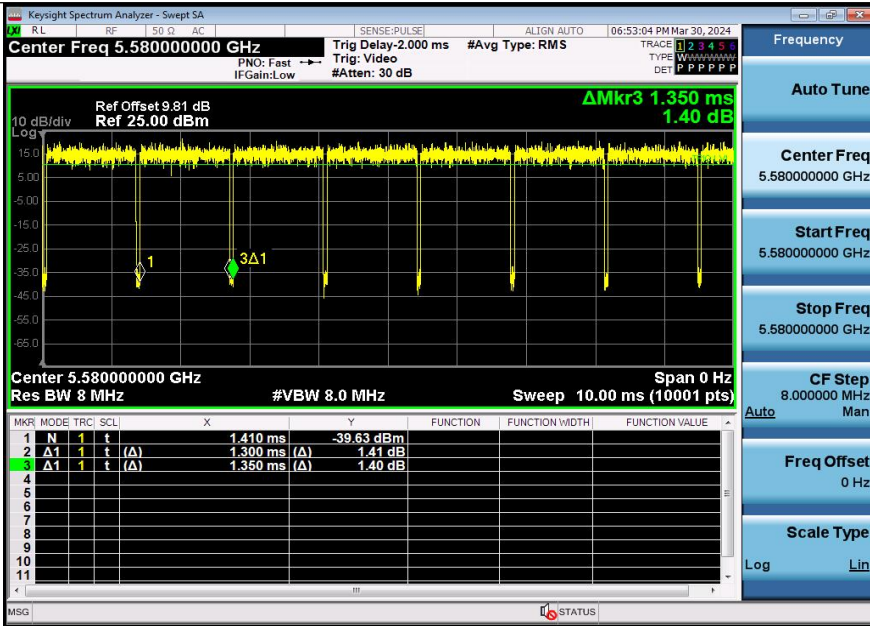
NTNV-11AC20SISO-Ant3-5580
