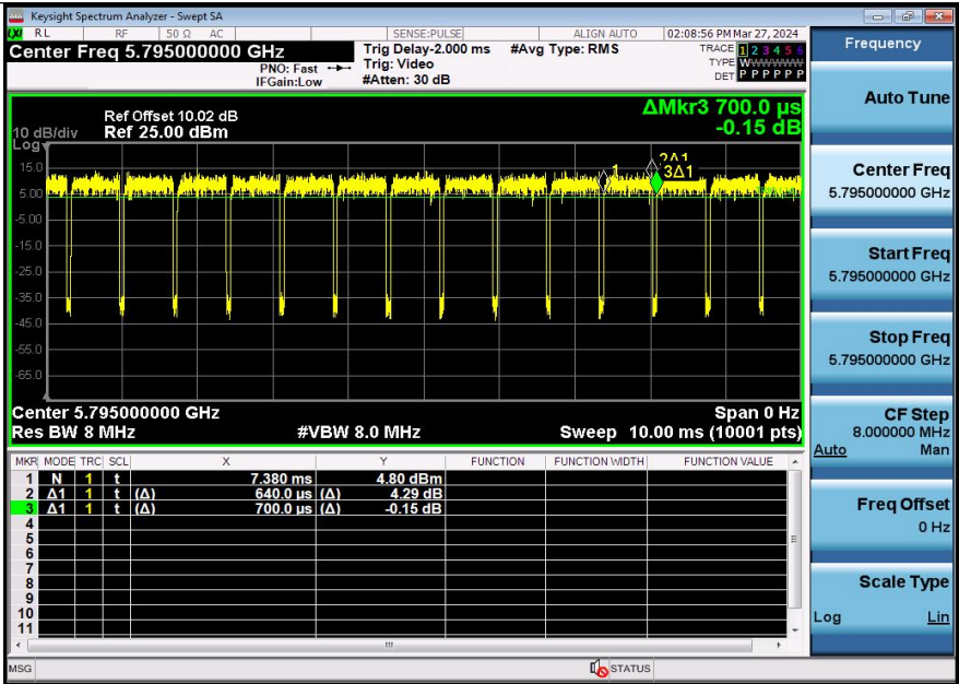
NTNV-11N40SISO-Ant3-5795
