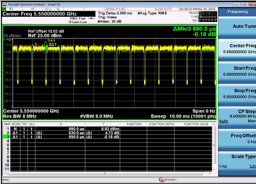
NTNV-11AC40SISO-Ant3-5550
