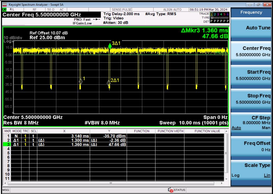
NTNV-11AC20SISO-Ant3-5500
