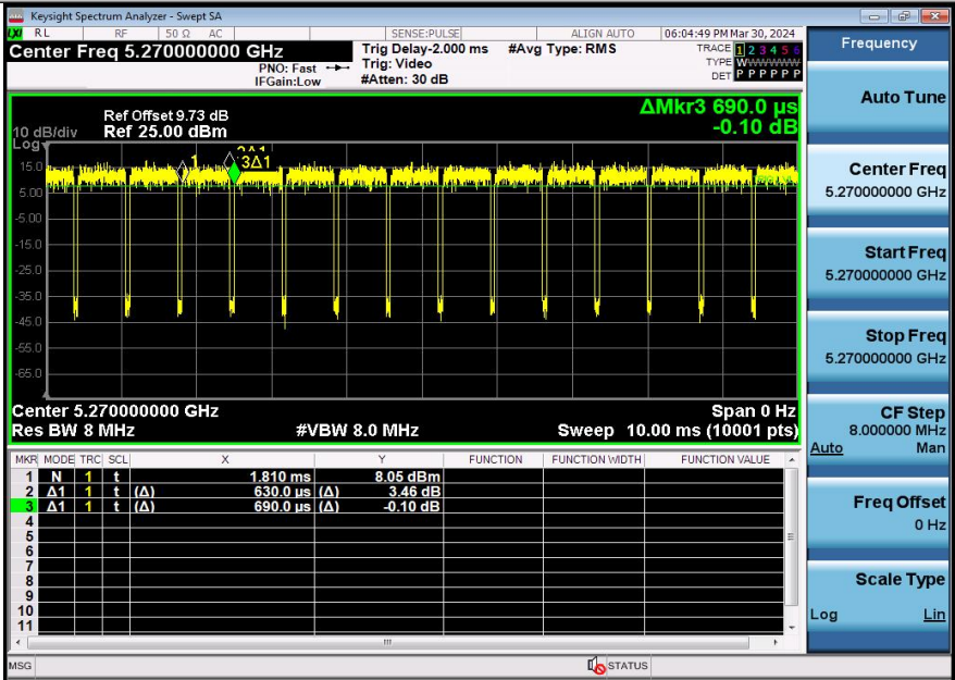
NTNV-11AC40SISO-Ant3-5270
