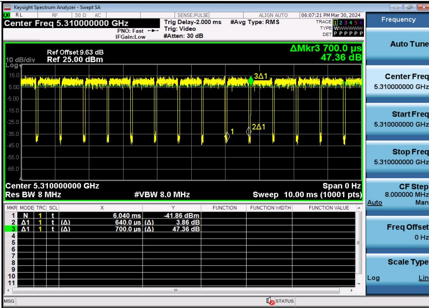
NTNV-11AC40SISO-Ant3-5310
