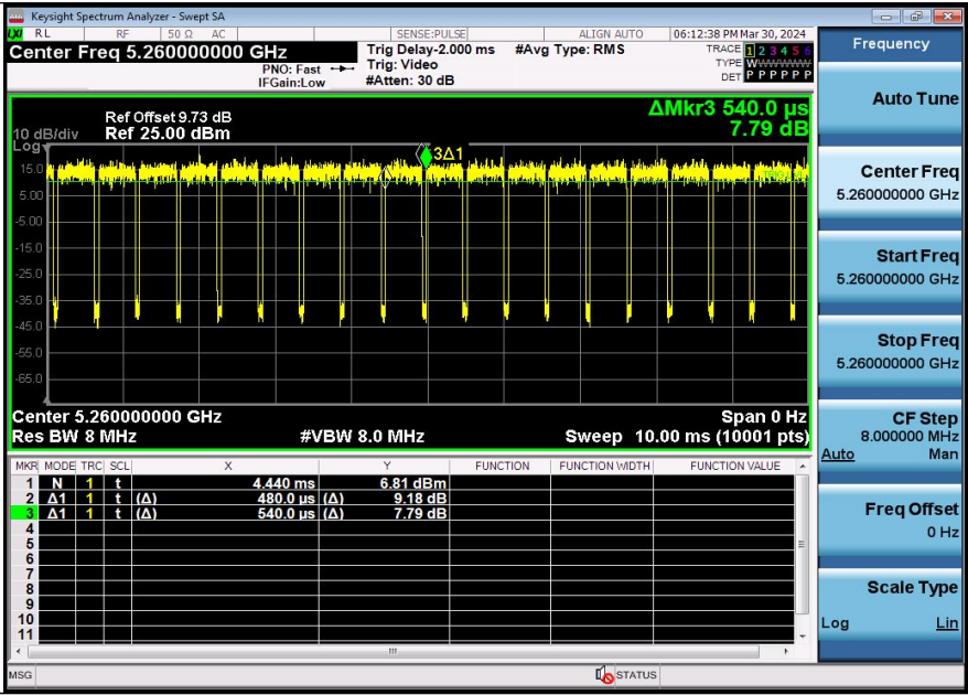
NTNV-11AX20SISO-Ant3-5260
