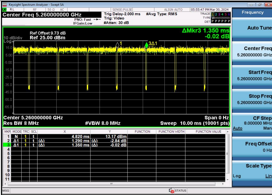
NTNV-11AC20SISO-Ant3-5260
