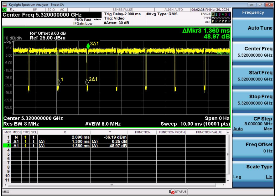
NTNV-11AC20SISO-Ant3-5320
