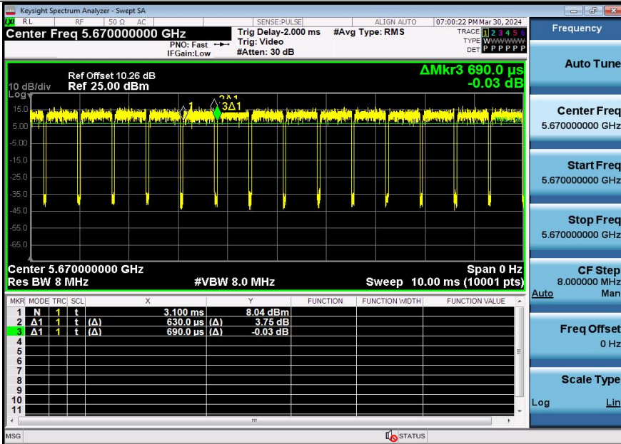
NTNV-11AC40SISO-Ant3-5670
