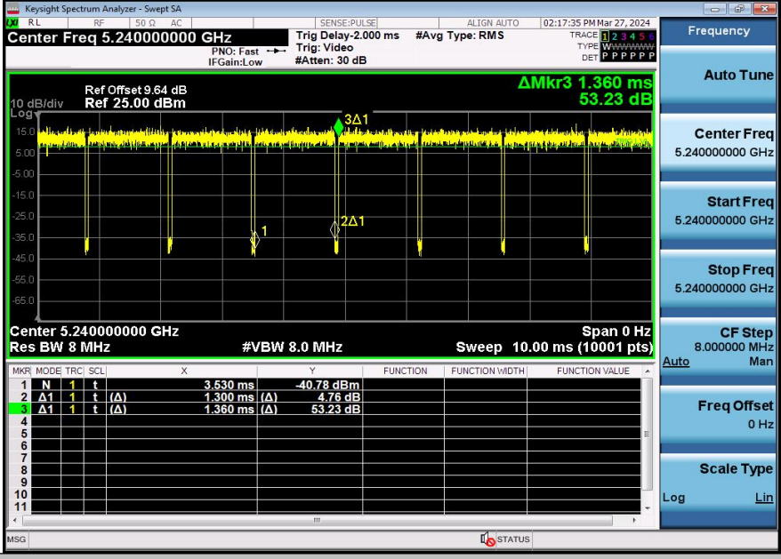
NTNV-11AC20SISO-Ant3-5240
