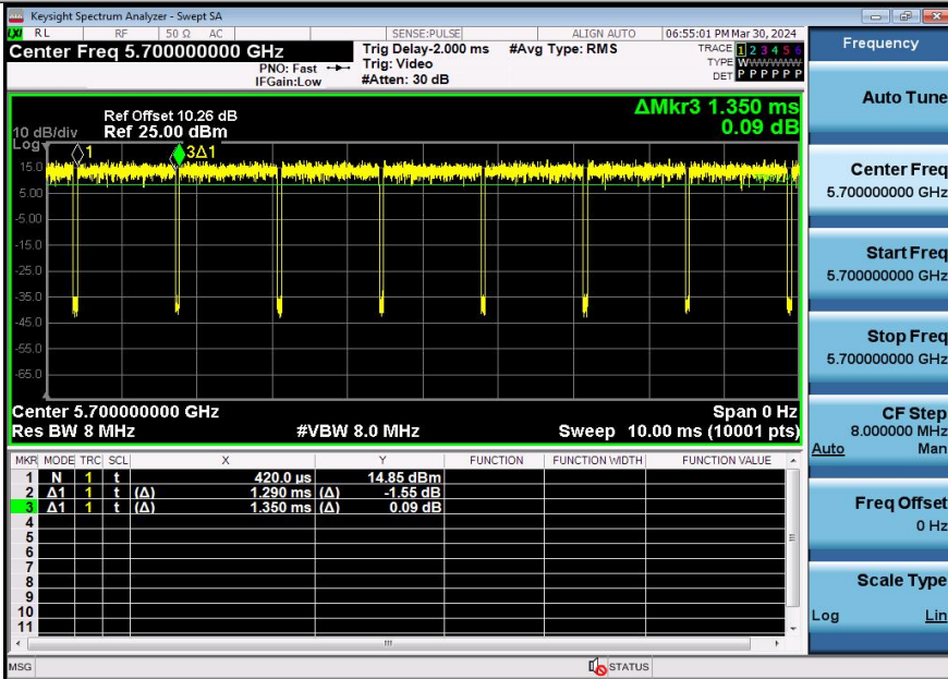
NTNV-11AC20SISO-Ant3-5700
