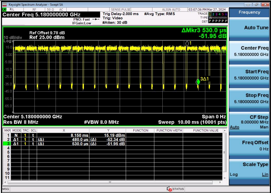
NTNV-11AX20SISO-Ant3-5180
