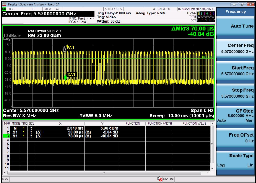
NTNV-11AC160SISO-Ant3-5570
