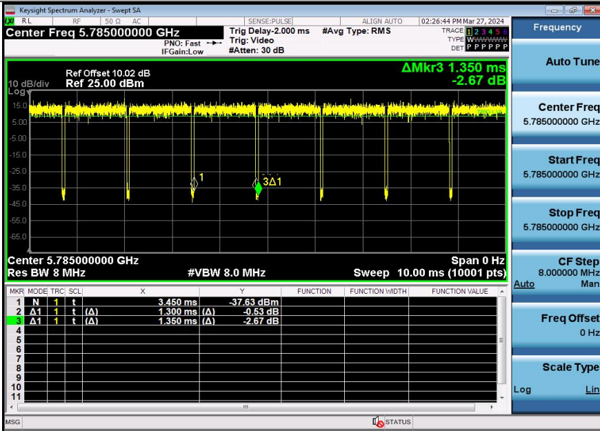
NTNV-11AC20SISO-Ant3-5785
