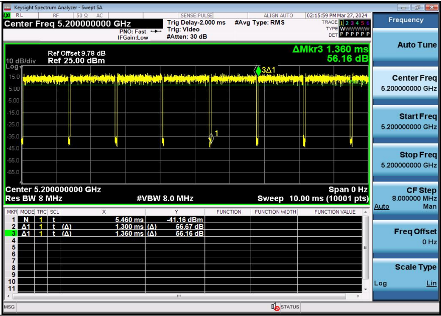
NTNV-11AC20SISO-Ant3-5200
