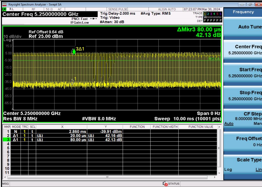
NTNV-11AC160SISO-Ant3-5250
