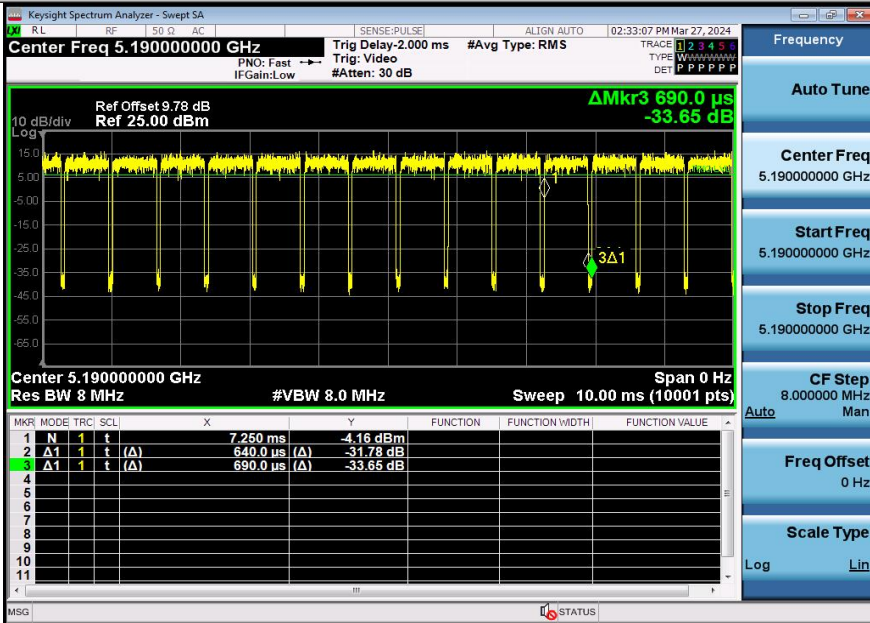
NTNV-11AC40SISO-Ant3-5190
