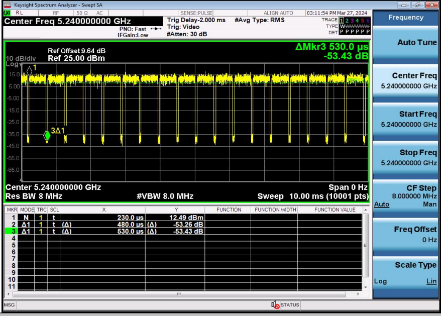
NTNV-11AX20SISO-Ant3-5240
