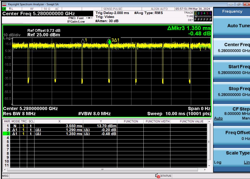
NTNV-11AC20SISO-Ant3-5280
