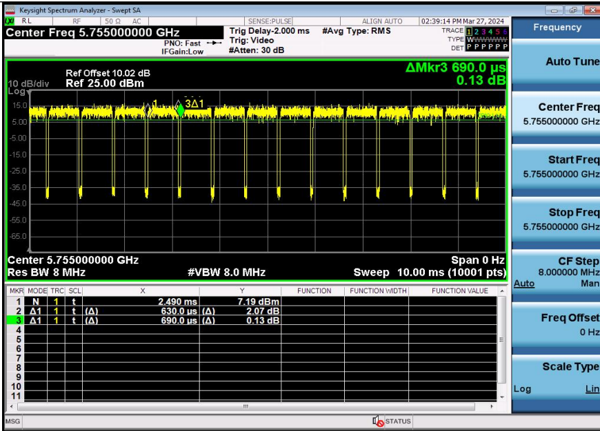
NTNV-11AC40SISO-Ant3-5755
