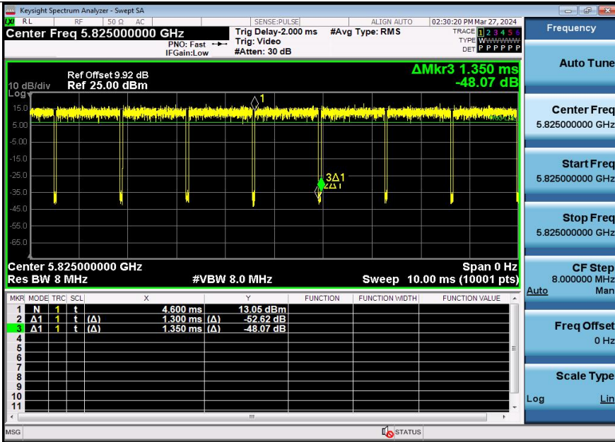
NTNV-11AC20SISO-Ant3-5825
