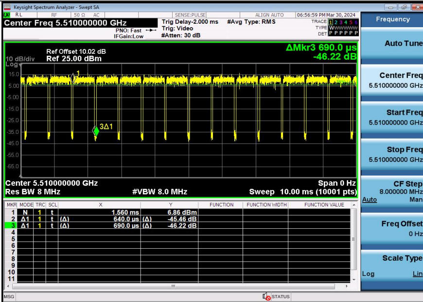
NTNV-11AC40SISO-Ant3-5510
