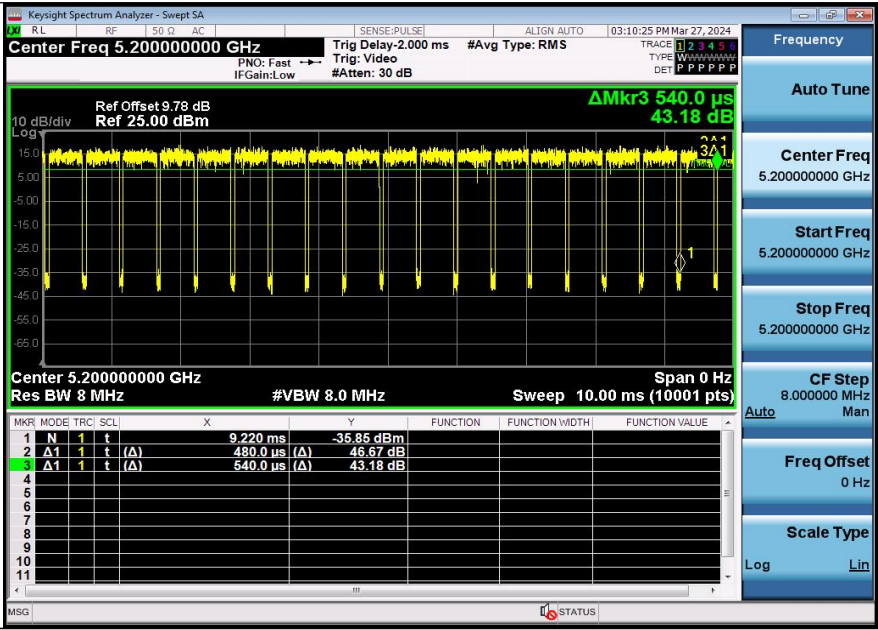
NTNV-11AX20SISO-Ant3-5200
