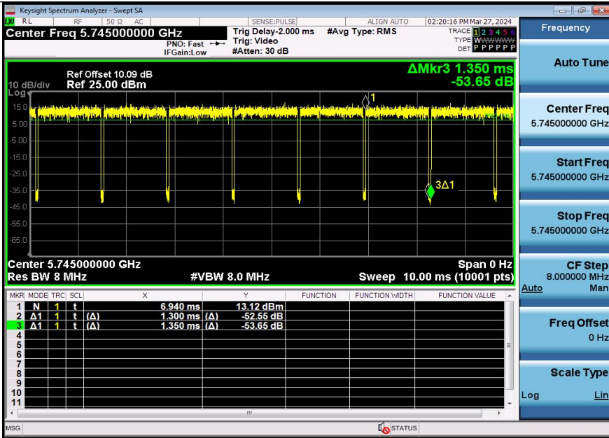
NTNV-11AC20SISO-Ant3-5745
