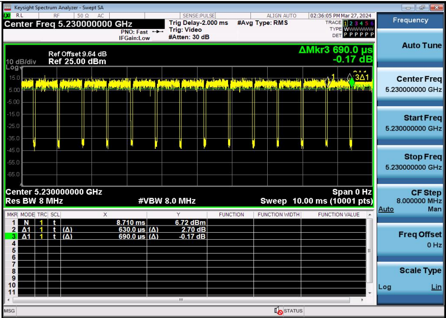
NTNV-11AC40SISO-Ant3-5230
