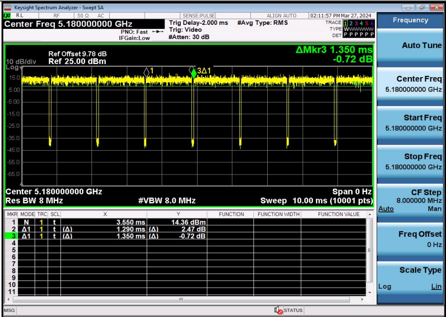
NTNV-11AC20SISO-Ant3-5180
