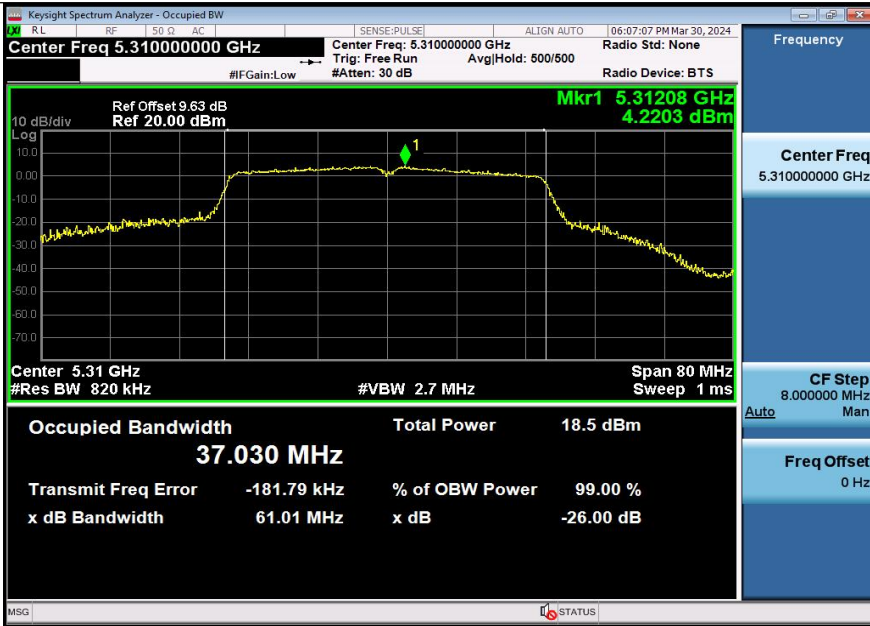
11AC40SISO-Ant3-5310
