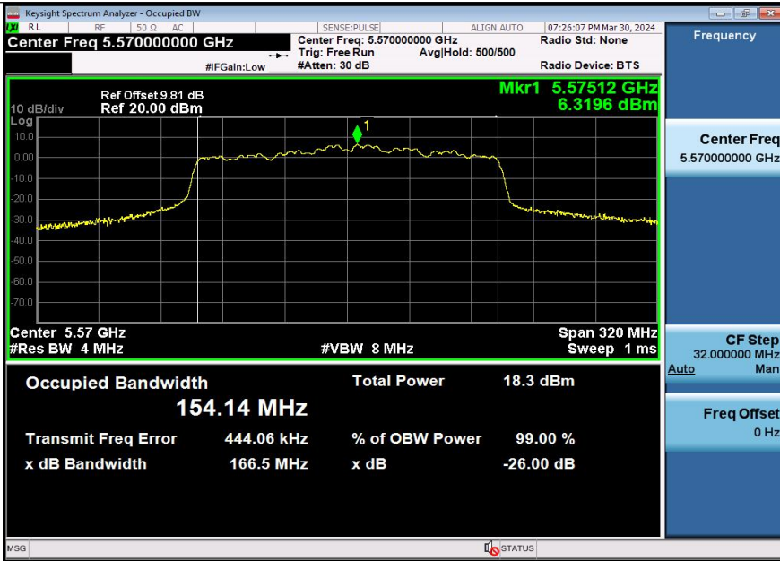
11AC160SISO-Ant3-5570
