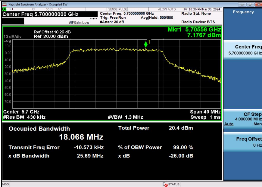
11AX20SISO-Ant3-5700
