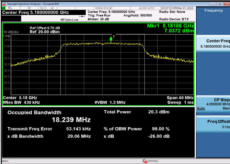
11AX20SISO-Ant3-5180
