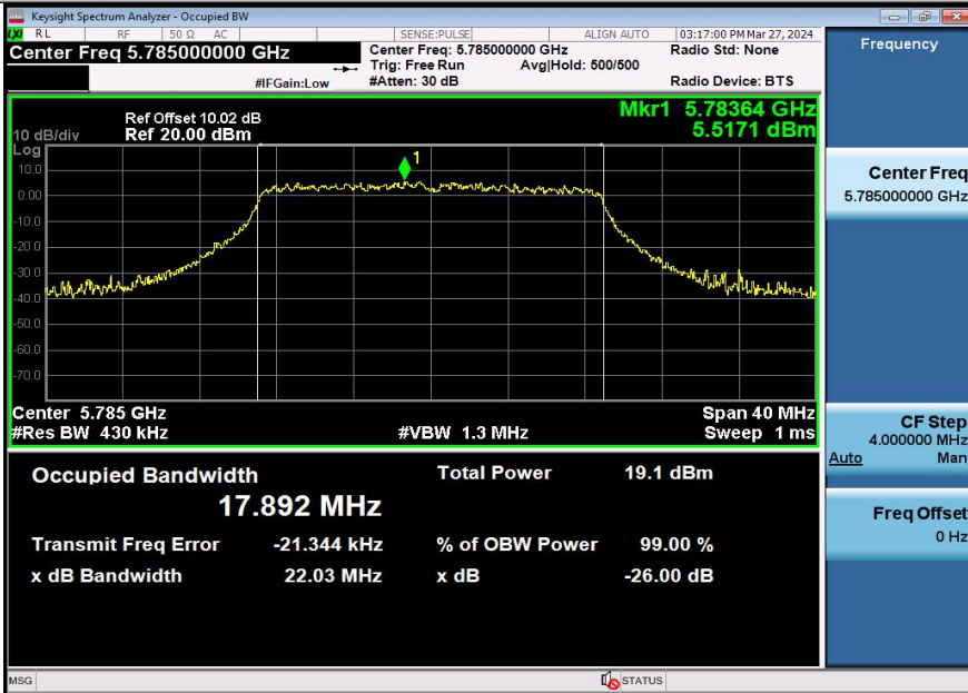
11AX20SISO-Ant3-5785
