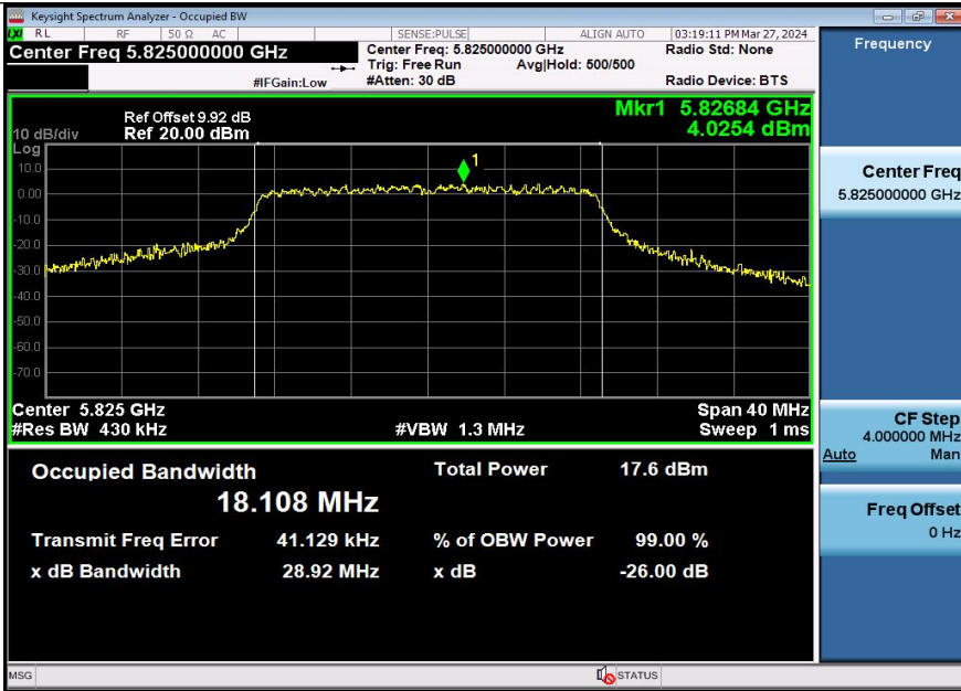
11AX20SISO-Ant3-5825
