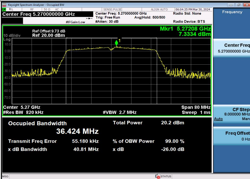
11AC40SISO-Ant3-5270
