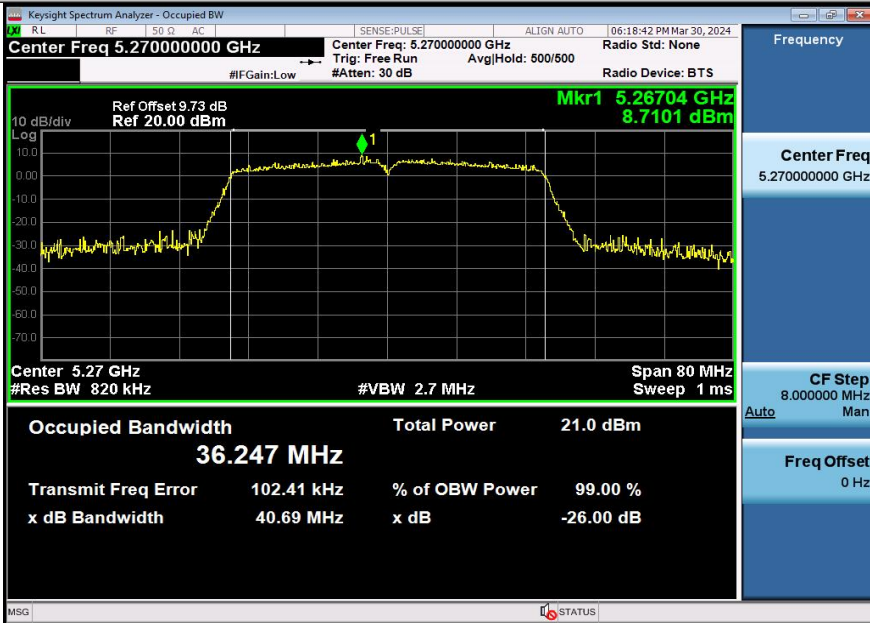
11AX40SISO-Ant3-5270
