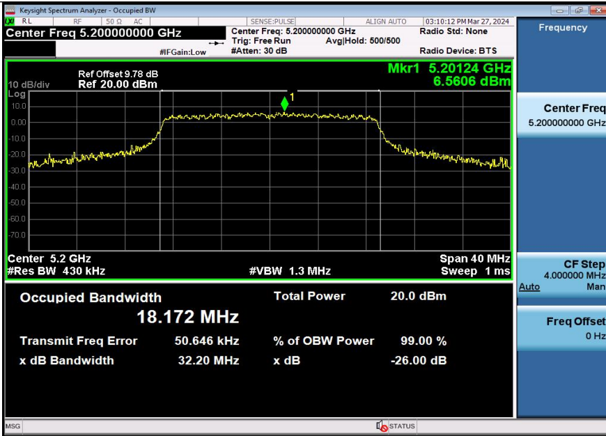
11AX20SISO-Ant3-5200
