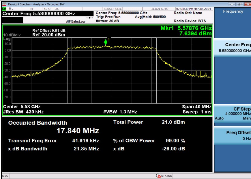
11AX20SISO-Ant3-5580
