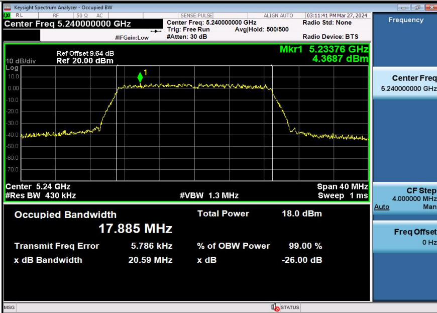
11AX20SISO-Ant3-5240
