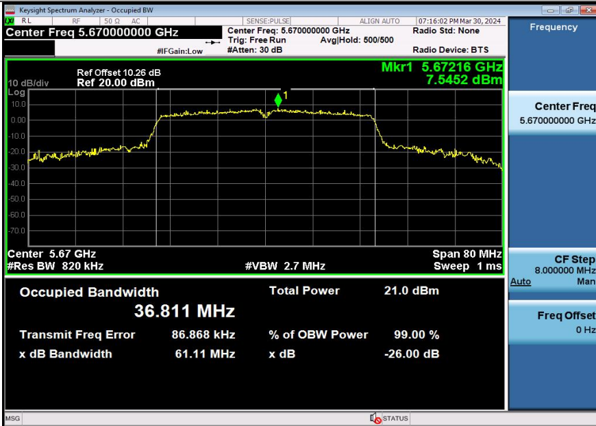
11AX40SISO-Ant3-5670
