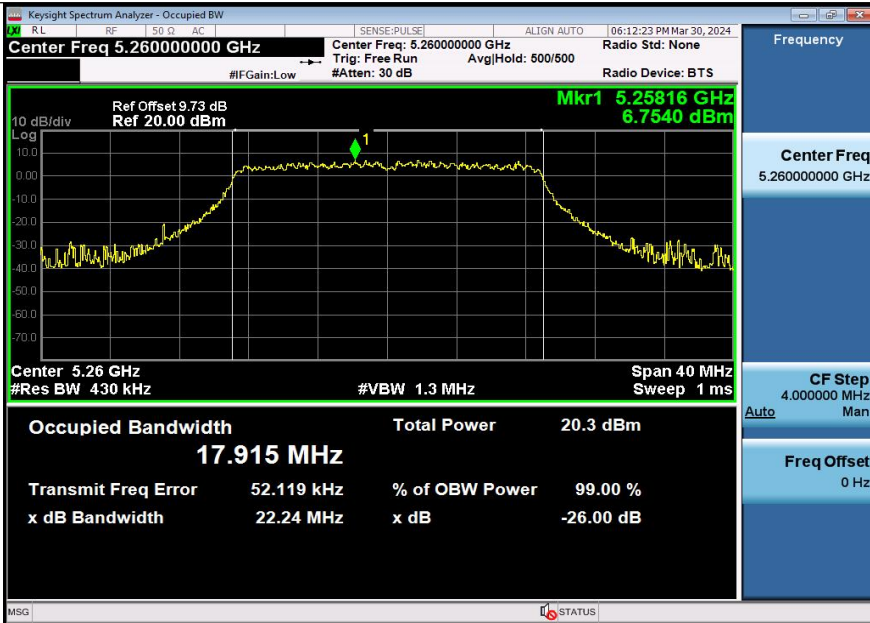
11AX20SISO-Ant3-5260
