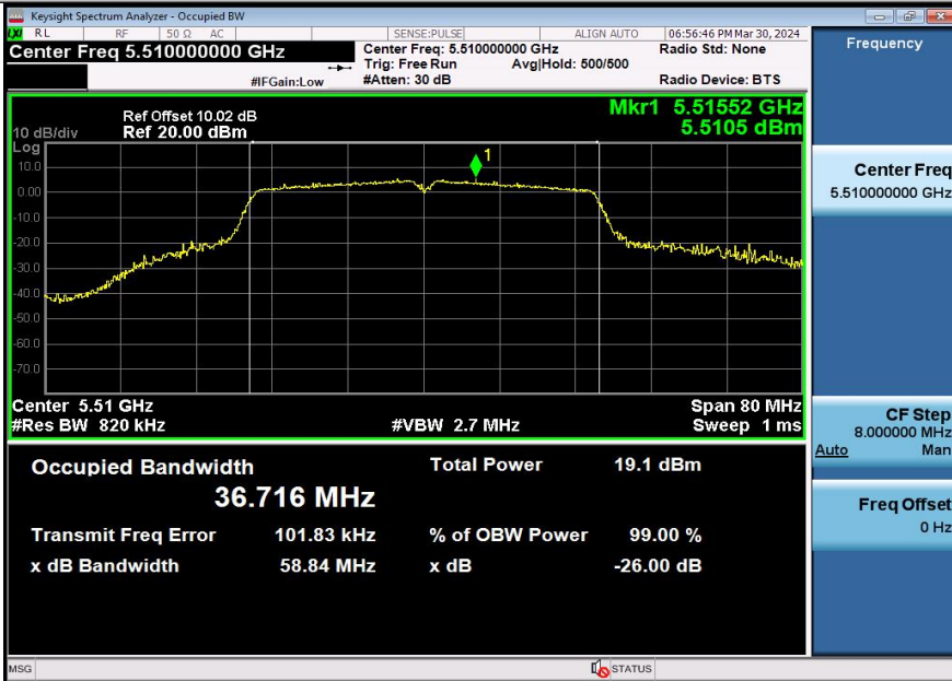
11AC40SISO-Ant3-5510
