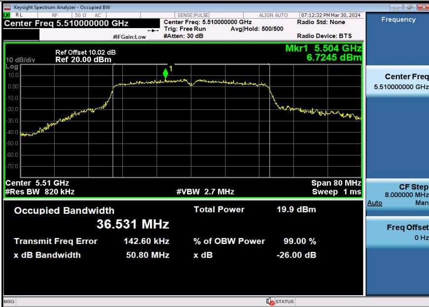
11AX40SISO-Ant3-5510
