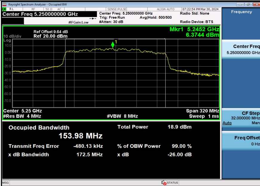
11AC160SISO-Ant3-5250
