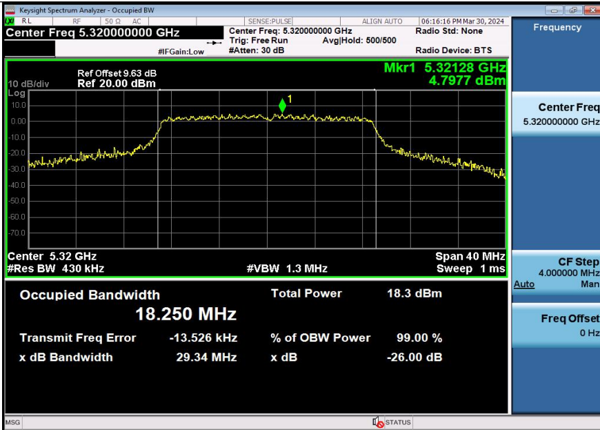
11AX20SISO-Ant3-5320
