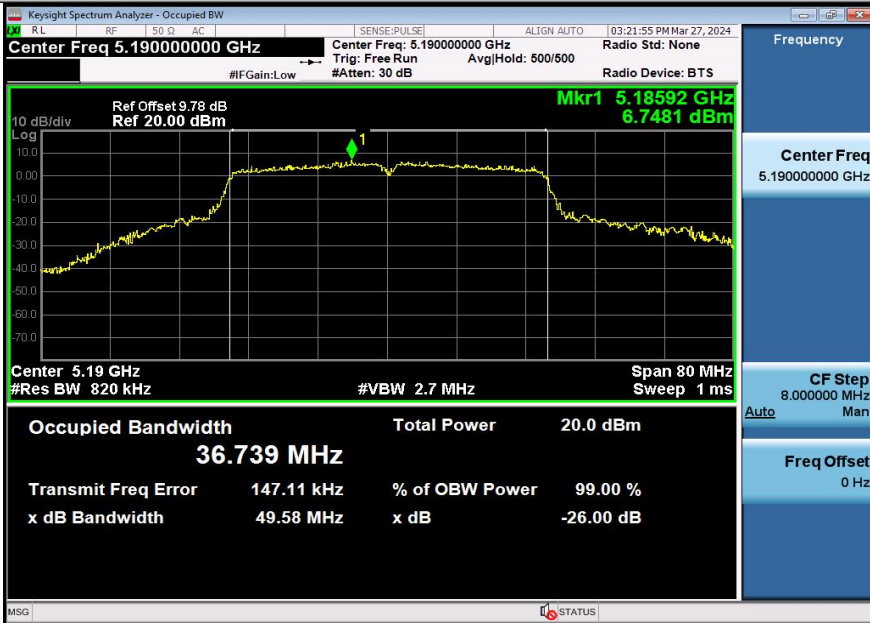
11AX40SISO-Ant3-5190
