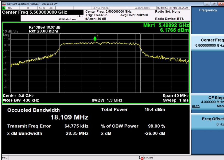
11AX20SISO-Ant3-5500
