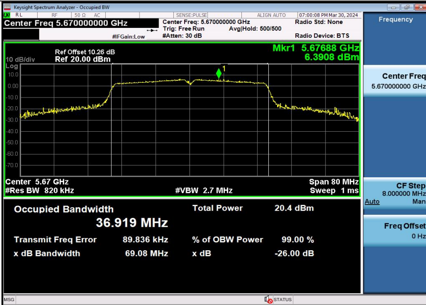
11AC40SISO-Ant3-5670
