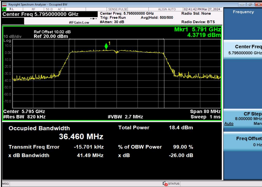
11AC40SISO-Ant3-5795
