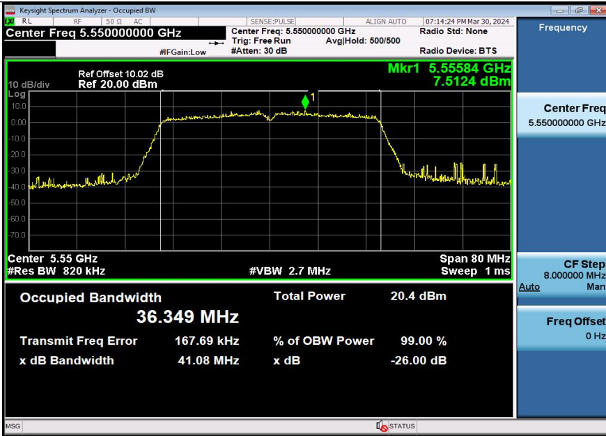
11AX40SISO-Ant3-5550
