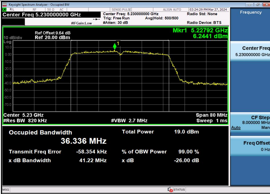
11AX40SISO-Ant3-5230
