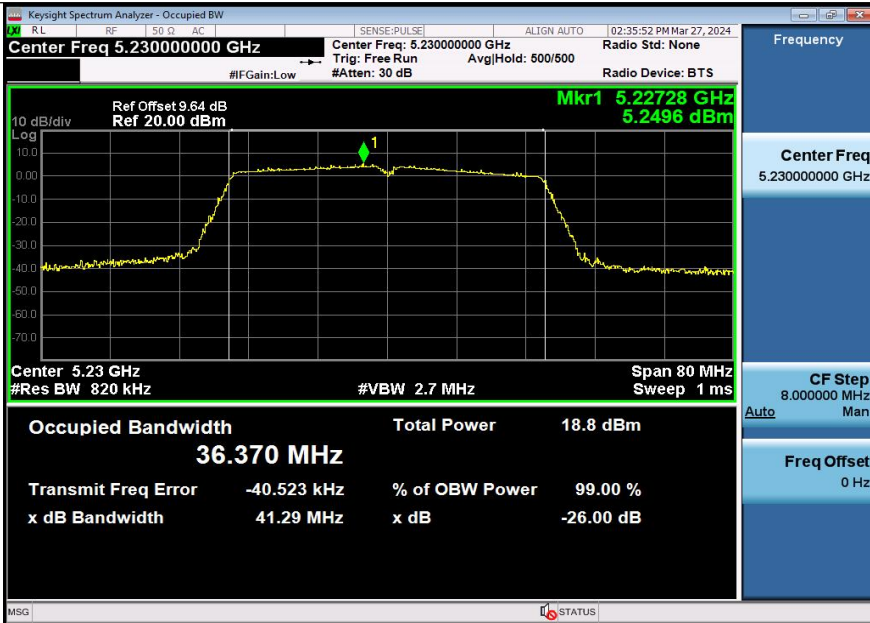
11AC40SISO-Ant3-5230
