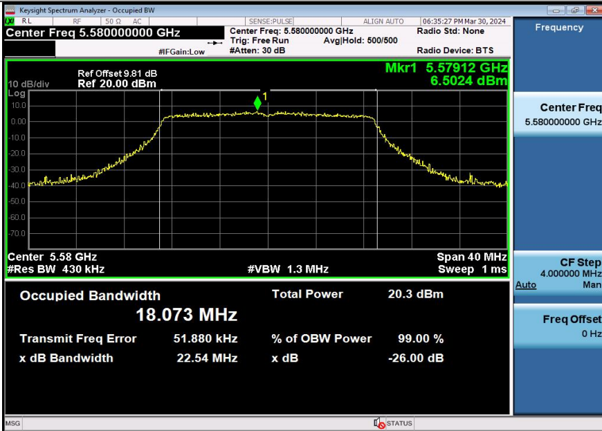
11N20SISO-Ant3-5580
