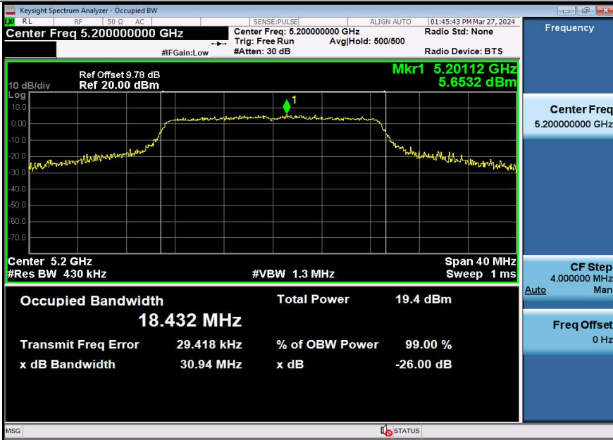
11N20SISO-Ant3-5200
