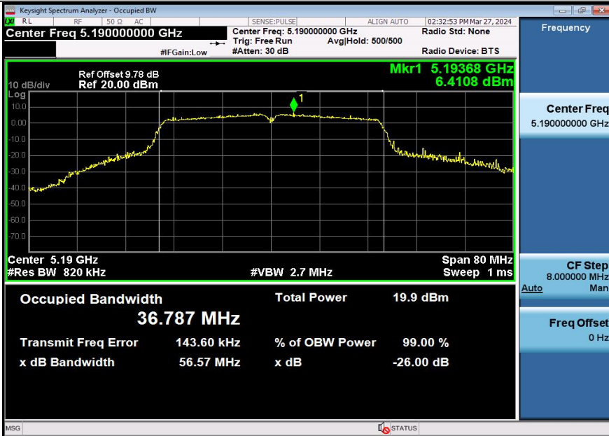
11AC40SISO-Ant3-5190
