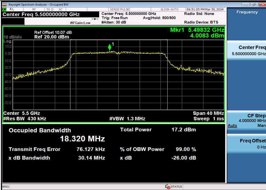
11AC20SISO-Ant3-5500
