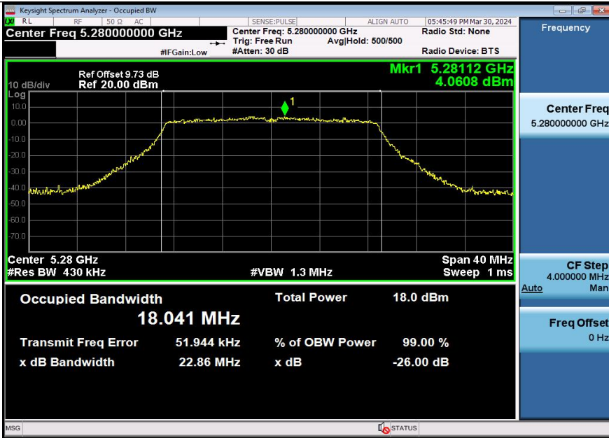
11N20SISO-Ant3-5280
