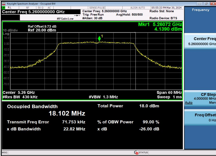
11AC20SISO-Ant3-5260
