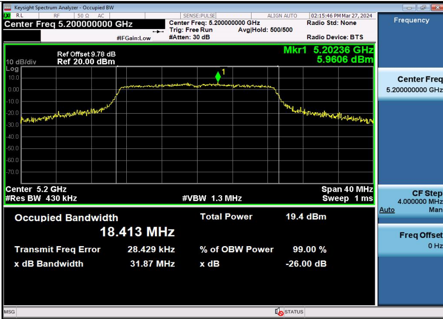
11AC20SISO-Ant3-5200
