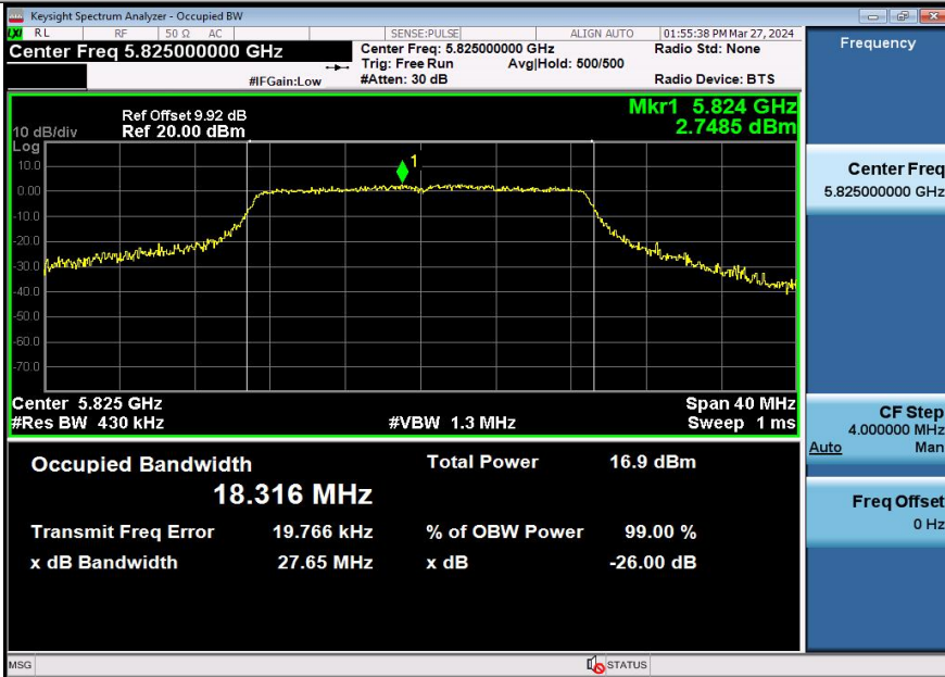
11N20SISO-Ant3-5825
