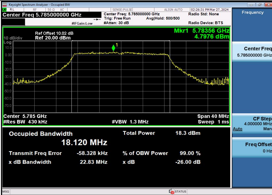
11AC20SISO-Ant3-5785
