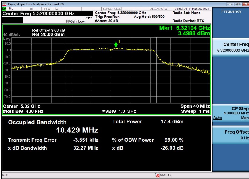
11AC20SISO-Ant3-5320
