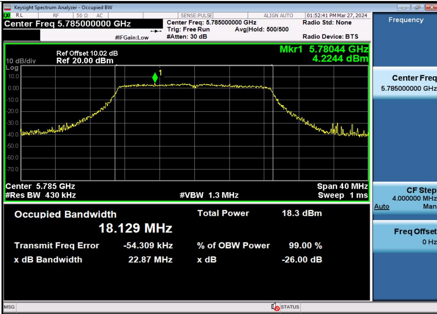
11N20SISO-Ant3-5785
