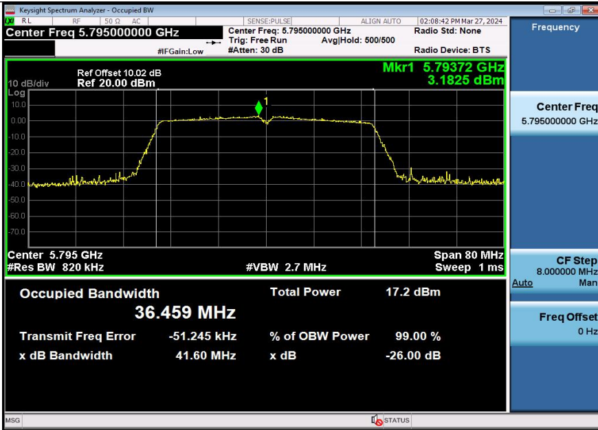
11N40SISO-Ant3-5795
