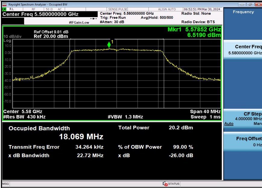
11AC20SISO-Ant3-5580
