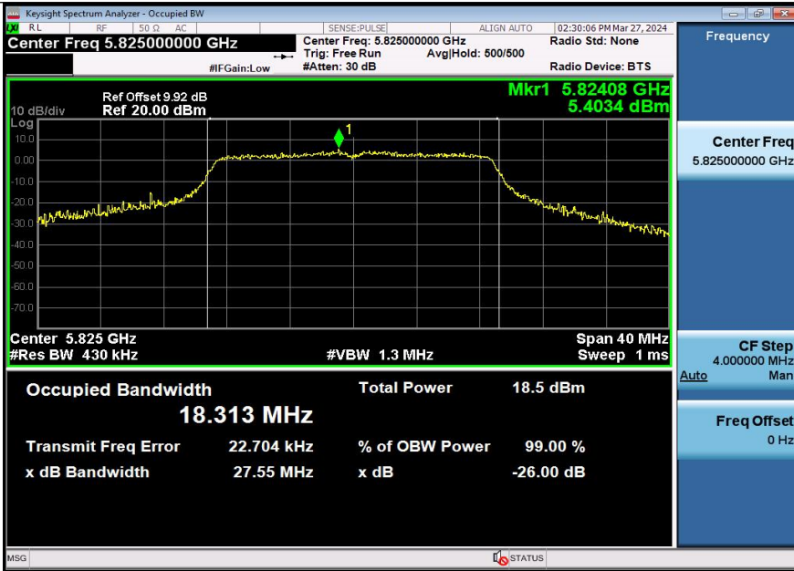
11AC20SISO-Ant3-5825
