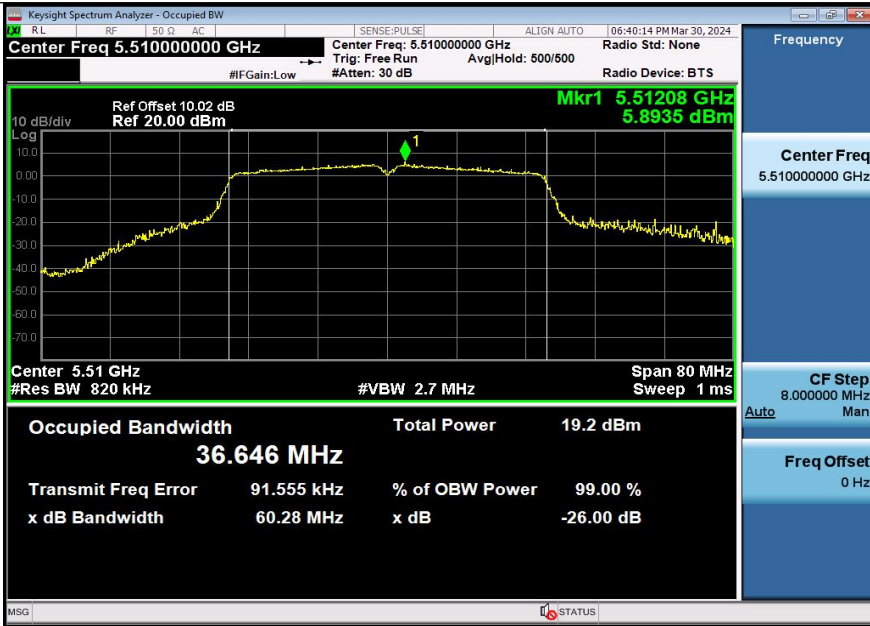
11N40SISO-Ant3-5510
