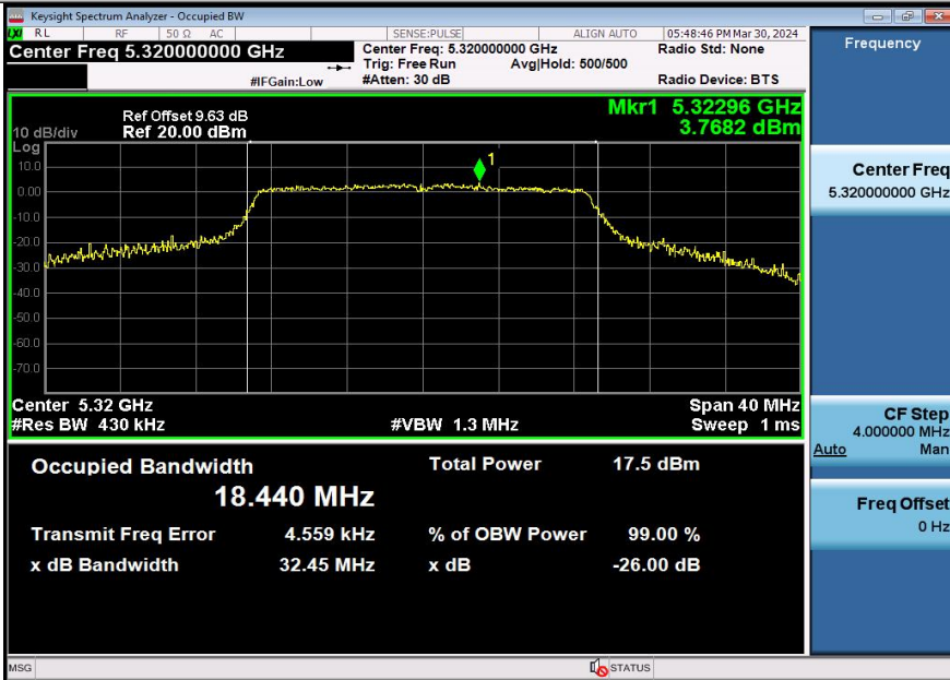
11N20SISO-Ant3-5320
