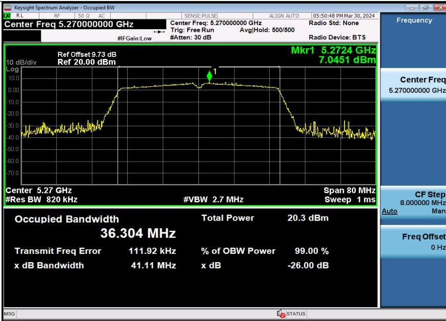
11N40SISO-Ant3-5270
