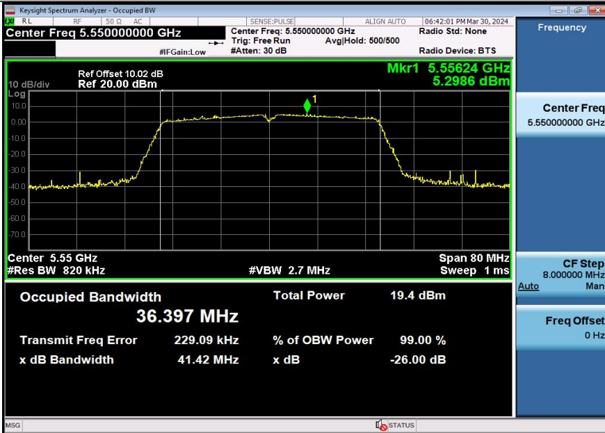
11N40SISO-Ant3-5550
