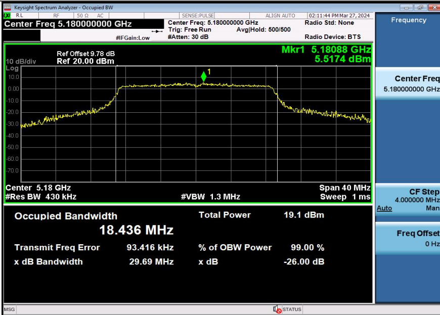
11AC20SISO-Ant3-5180
