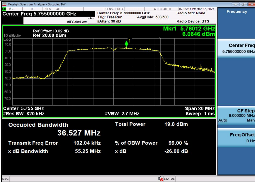
11N40SISO-Ant3-5755
