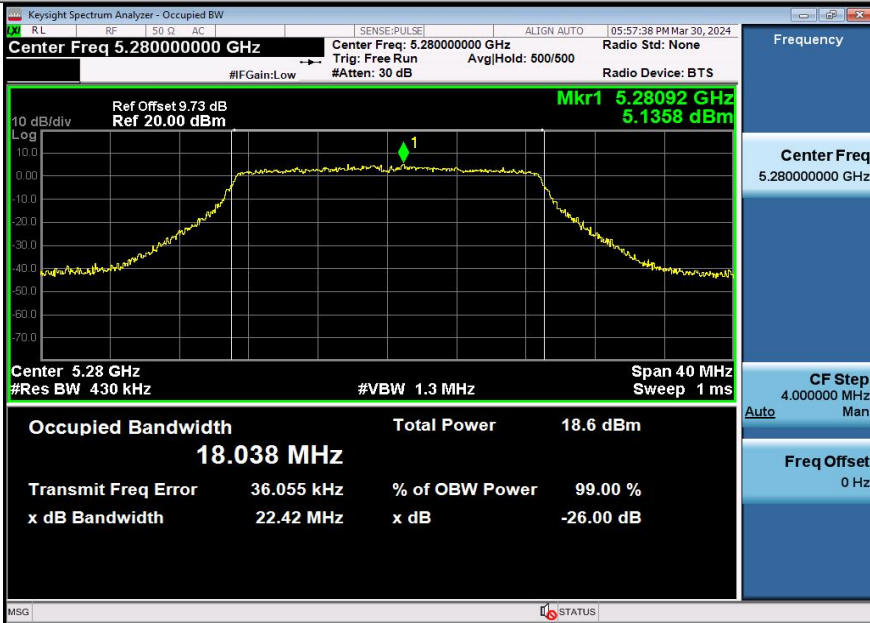
11AC20SISO-Ant3-5280
