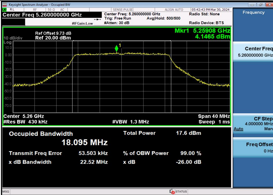
11N20SISO-Ant3-5260
