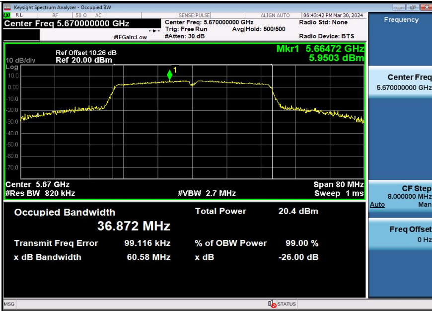
11N40SISO-Ant3-5670
