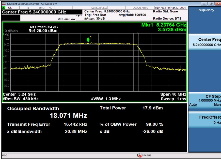
11N20SISO-Ant3-5240
