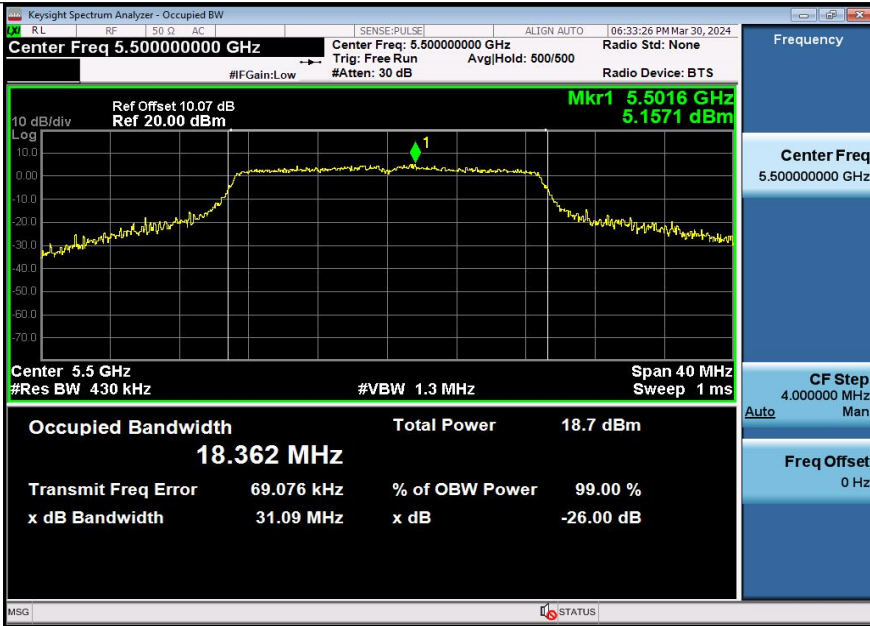
11N20SISO-Ant3-5500
