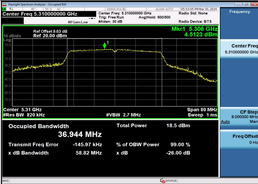
11N40SISO-Ant3-5310
