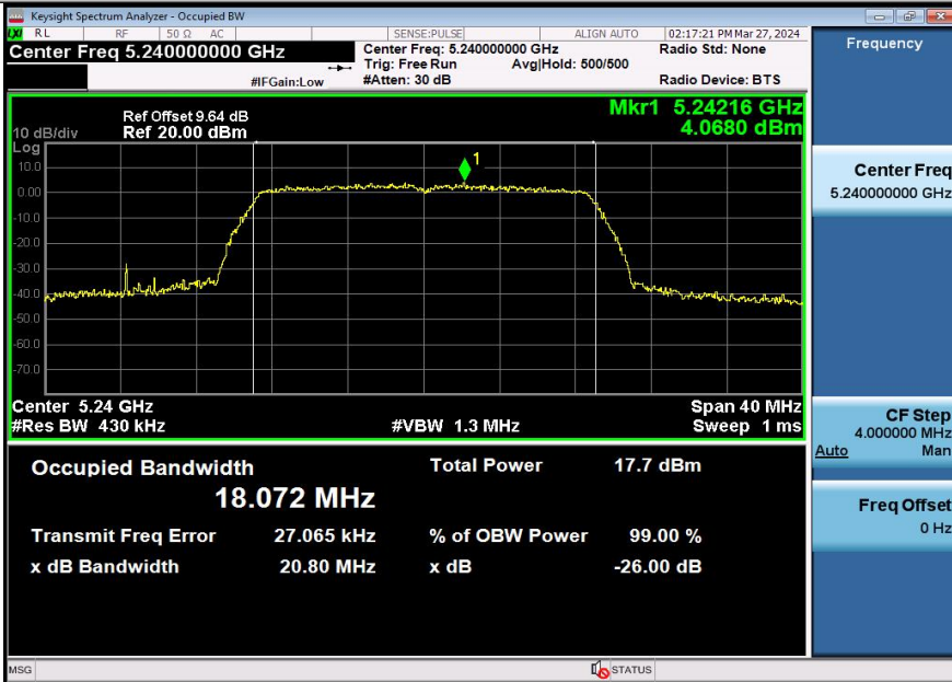
11AC20SISO-Ant3-5240
