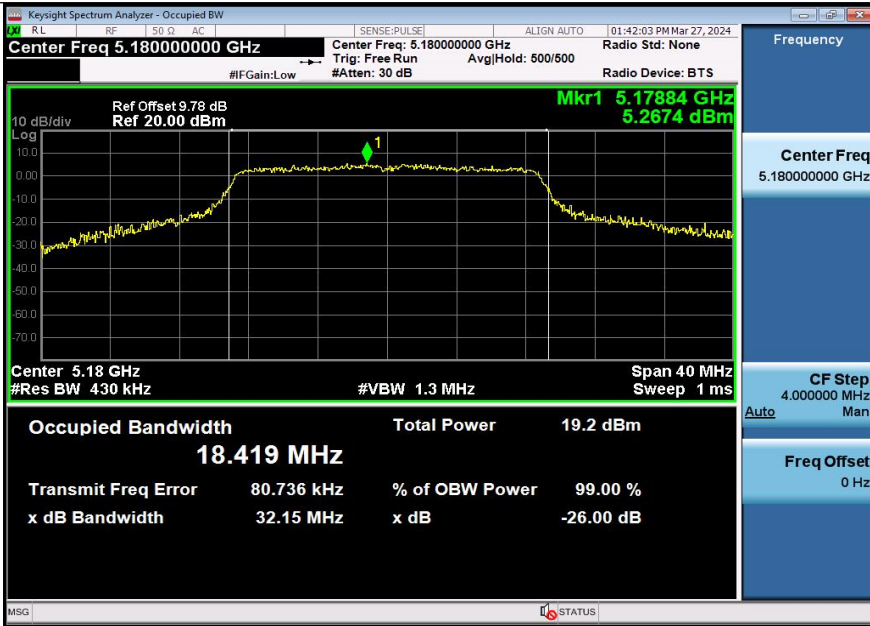
11N20SISO-Ant3-5180
