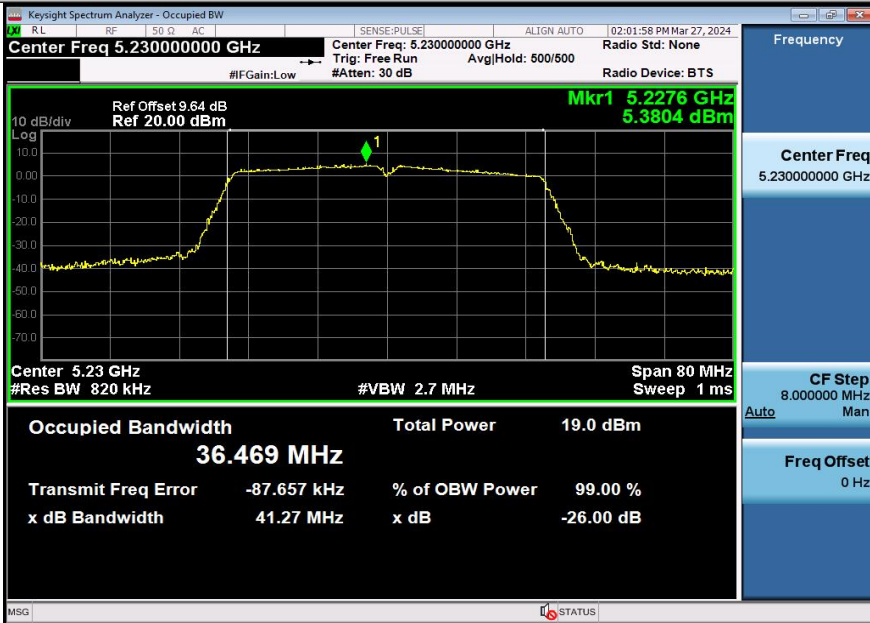
11N40SISO-Ant3-5230
