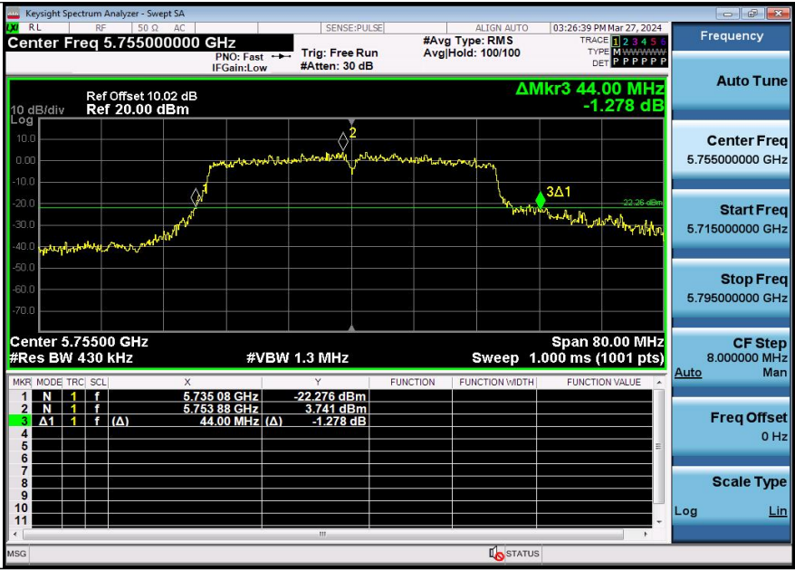
11AX40SISO-Ant3-5755
