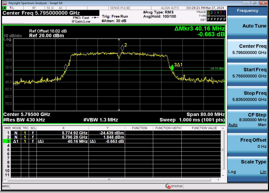
11AX40SISO-Ant3-5795
