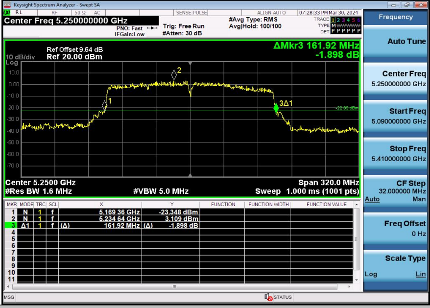
11AX160SISO-Ant3-5250
