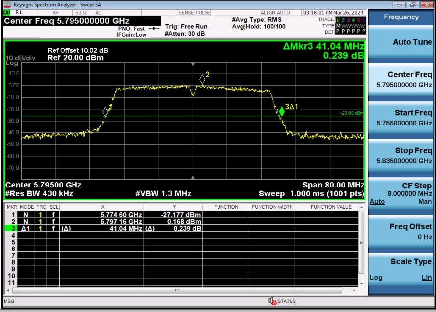
11AX40SISO-Ant1-5795
