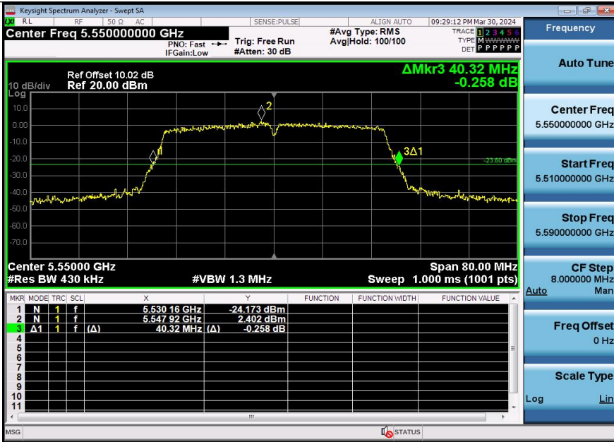
11AX40SISO-Ant1-5550
