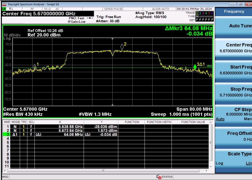
11AX40SISO-Ant1-5670
