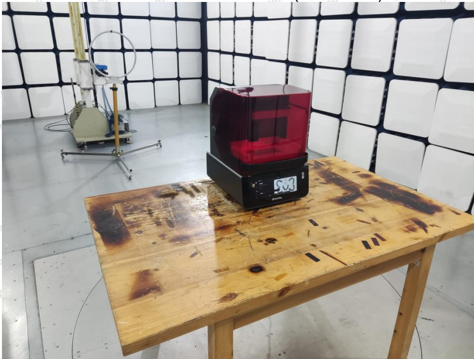
Undesirable emission limits (9KHz- 30M)
