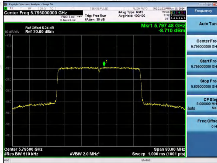
11AX40MIMO-Ant2-5795-PASS
