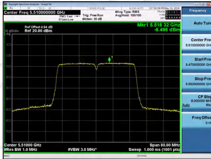
11N40MIMO-Ant2-5510-PASS
