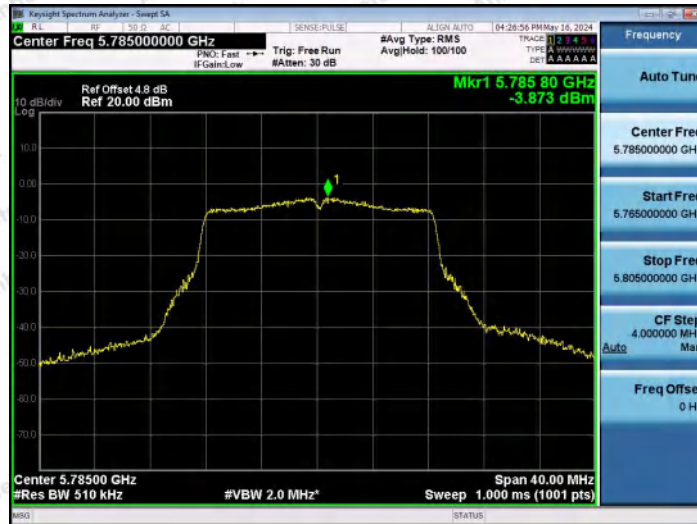
11A-Ant2-5785-PASS
