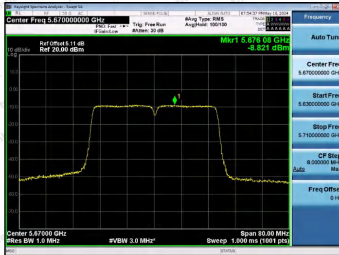
11AC40MIMO-Ant1-5670-PASS
