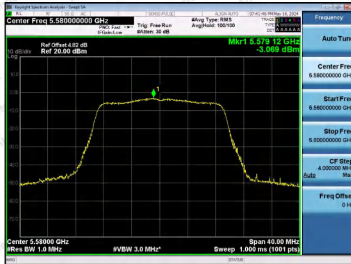
11AC20MIMO-Ant2-5580-PASS
