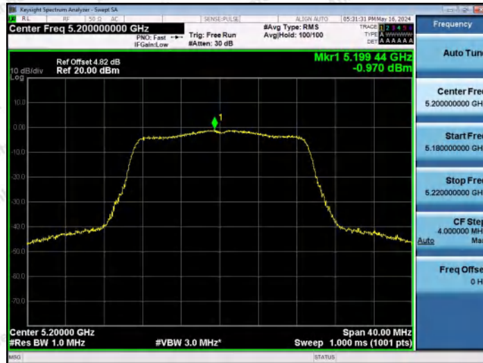
11N20MIMO-Ant2-5200-PASS
