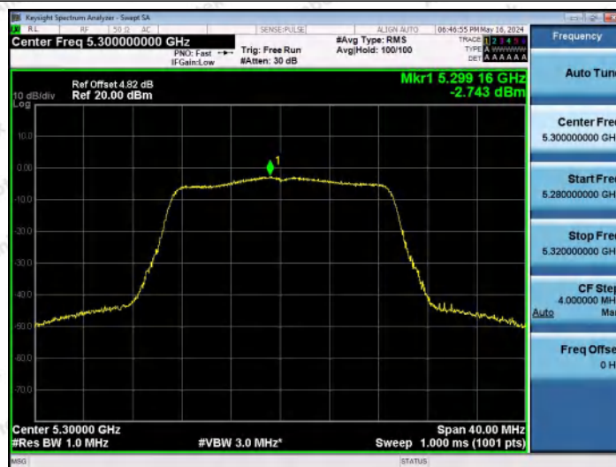
11AC20MIMO-Ant1-5300-PASS
