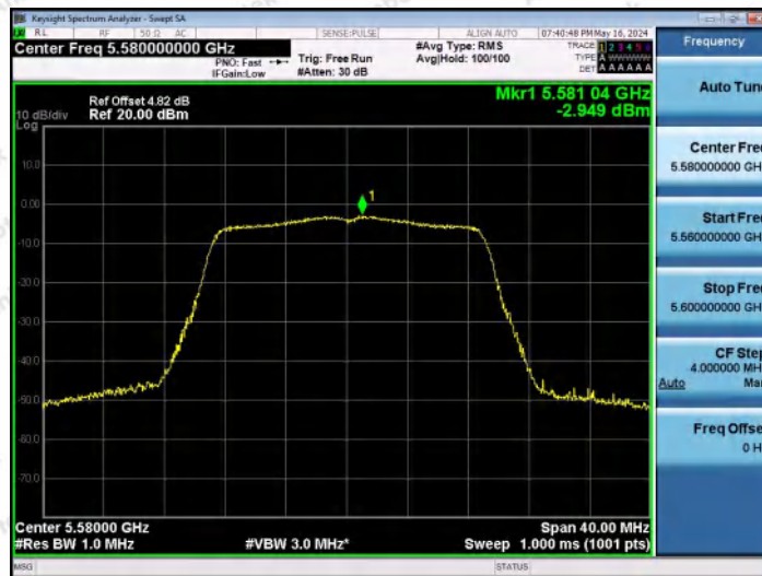
11AC20MIMO-Ant1-5580-PASS
