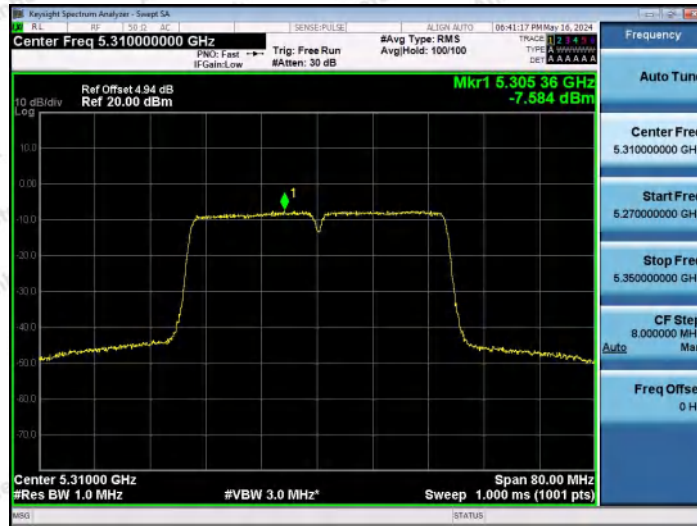
11N40MIMO-Ant1-5310-PASS
