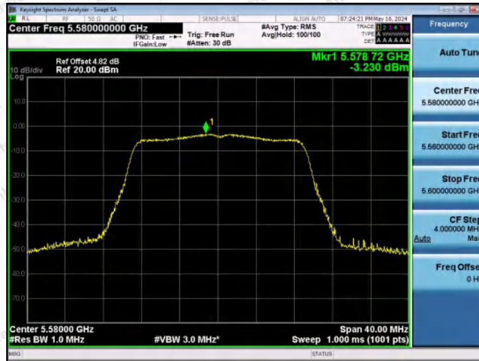
11N20MIMO-Ant2-5580-PASS
