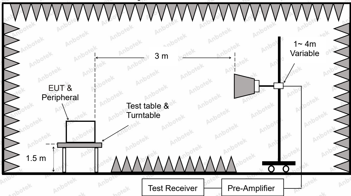
Figure 3. Above 1 GHz
