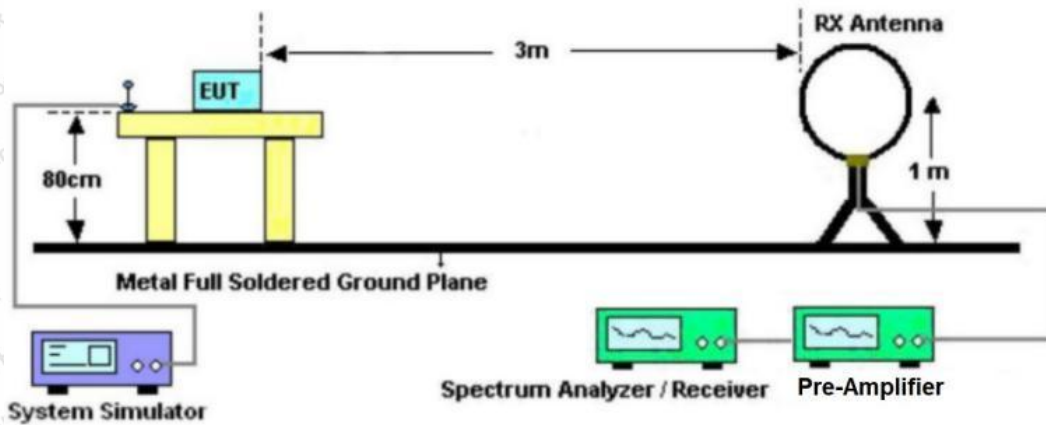
Figure 1. Below 30MHz
