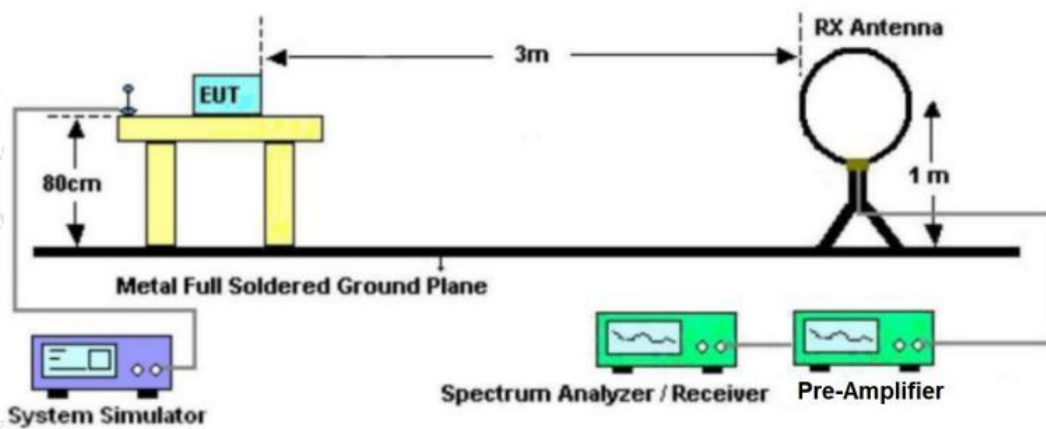
Figure 1. Below 30MHz
