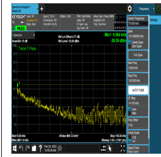
NTNV_DC_5A_n41A_PC3_30_5+60_M+M_TID17 _NS_01_0.009_0.15_#1
