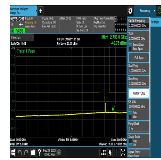
NTNV_DC_5A_n41A_PC3_30_5+60_M+M_TID17 _NS_01_0.15_30_#1
