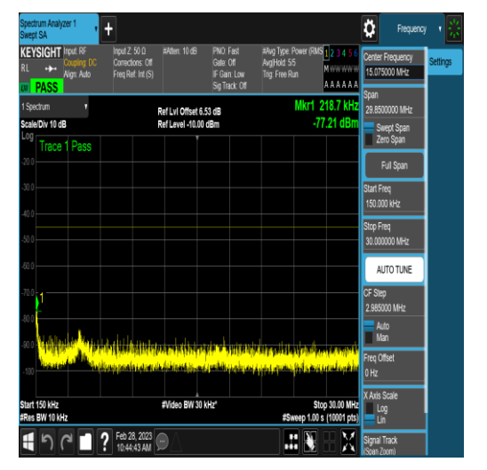
NTNV_DC_5A_n41A_PC3_30_5+60_M+L_TID18 _NS_01_0.15_30_#1
