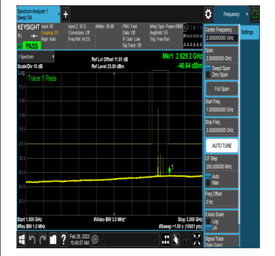
NTNV_DC_5A_n41A_PC3_30_5+60_M+L_TID16 _NS_01_1000_3000_#1
