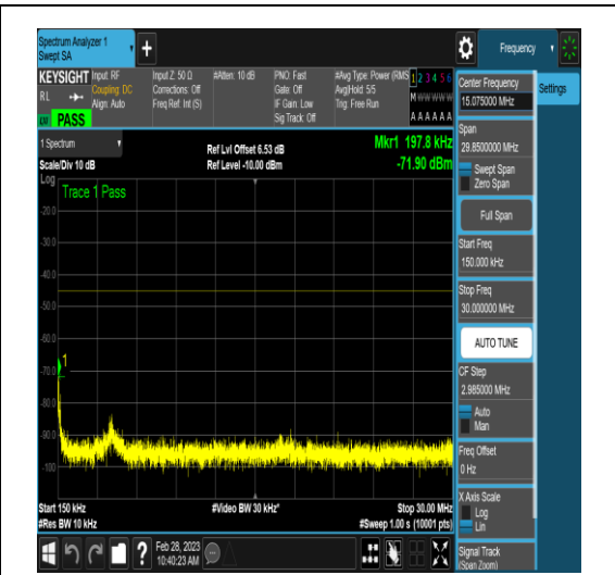
NTNV_DC_5A_n41A_PC3_30_5+60_M+L_TID16 _NS_01_0.15_30_#1
