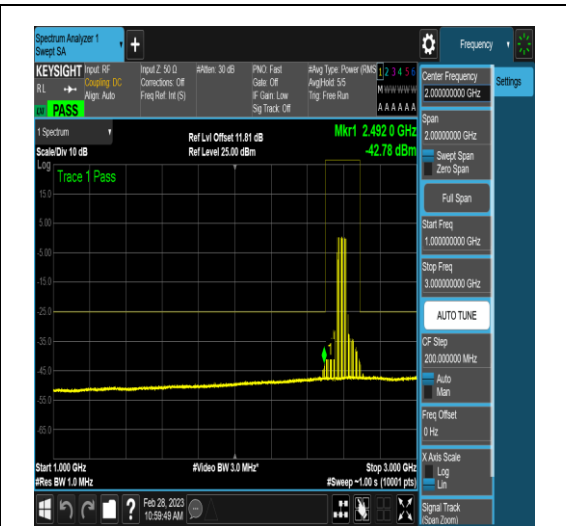
NTNV_DC_5A_n41A_PC3_30_5+60_M+M_TID18 _NS_01_1000_3000_#1
