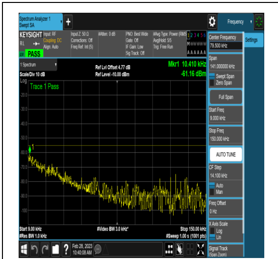
NTNV_DC_5A_n41A_PC3_30_5+60_M+L_TID16 _NS_01_0.009_0.15_#1
