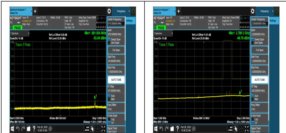
NTNV_DC_5A_n41A_PC3_30_5+60_M+L_TID5_ NS_01_30_1000_#1
