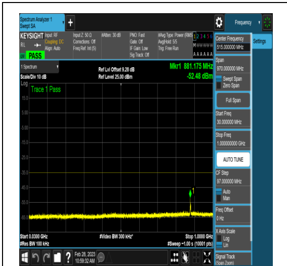
NTNV_DC_5A_n41A_PC3_30_5+60_M+M_TID18 _NS_01_30_1000_#1
