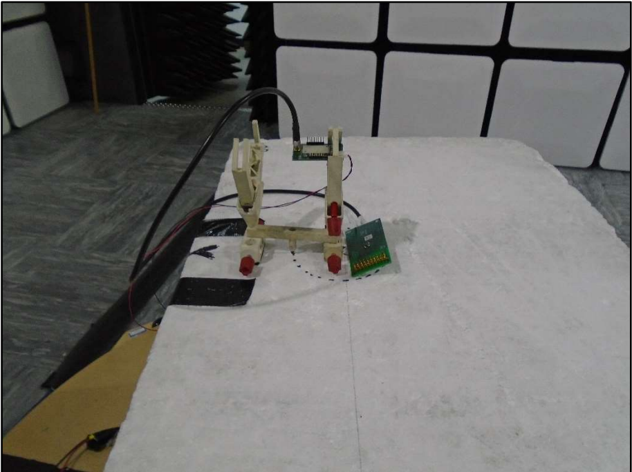
Figure 3 - Coil Antenna, Orientation X
