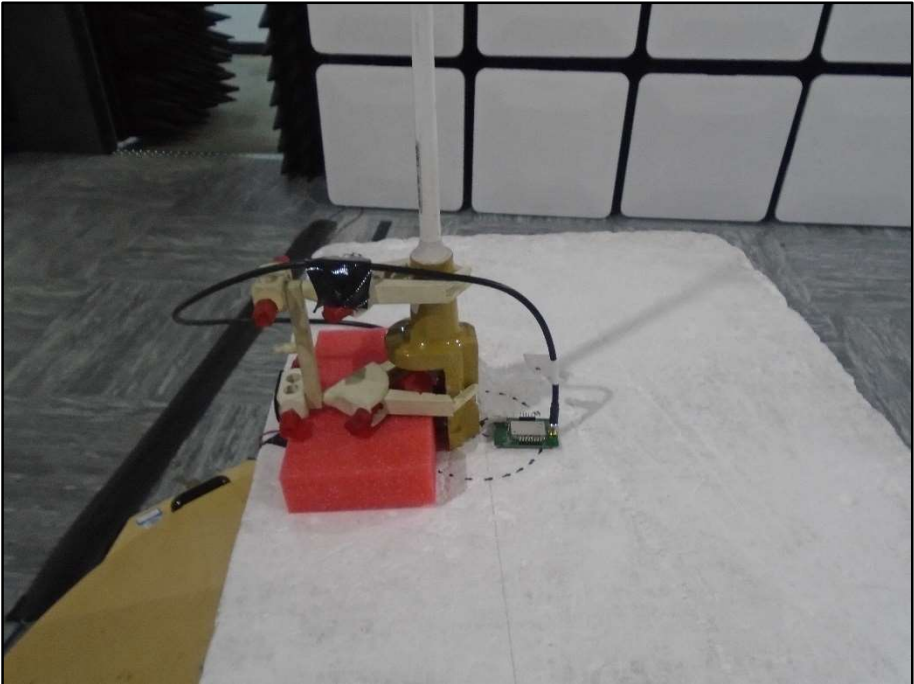
Figure 8 - Dipole Stick Antenna, Orientation X
