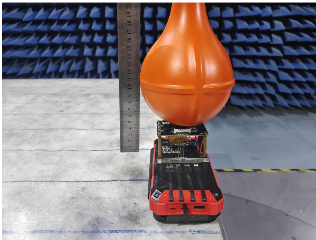
H-Field &amp; E-Field Strength_ Position A
