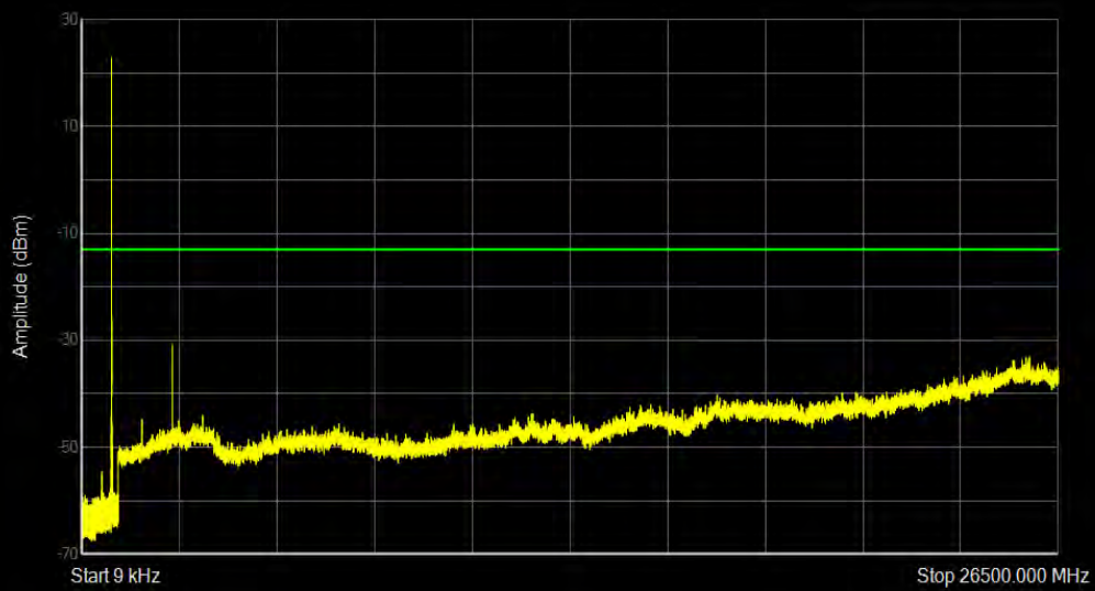
Band5 16QAM BW=5MHz Channel=20425 RB Size=1 Position=#0
