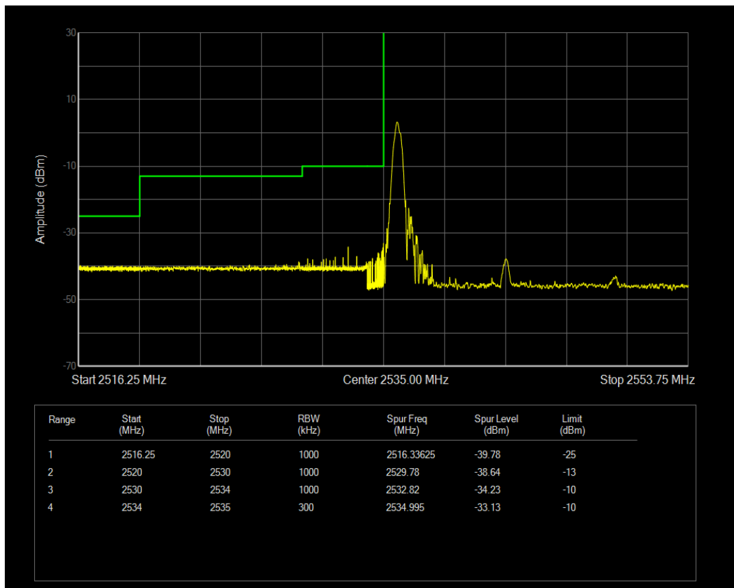
Band41(2535-2655) QAM16 BW=15MHz Channel=40115 RB Size=1 Position=#Max
