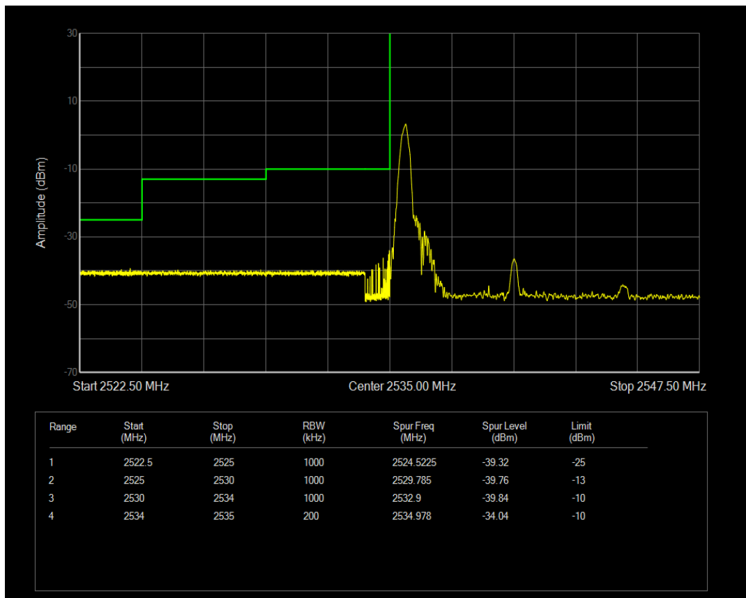
Band41(2535-2655) QAM16 BW=10MHz Channel=40090 RB Size=1 Position=#Max
