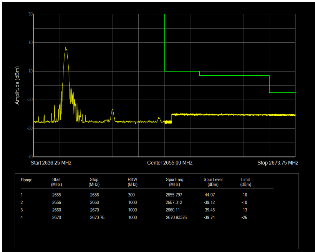
Band41(2535-2655) QAM16 BW=15MHz Channel=41165 RB Size=1 Position=#Max
