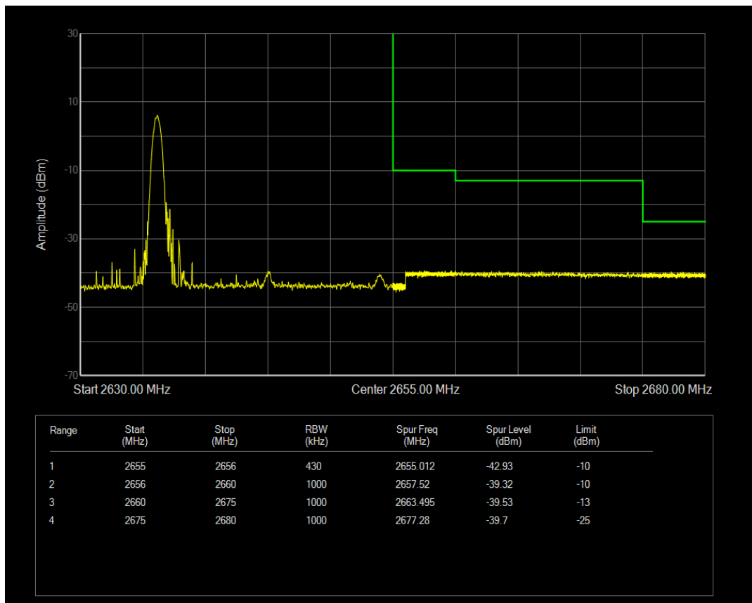
Band41(2535-2655) QAM16 BW=20MHz Channel=41140 RB Size=1 Position=#Max
