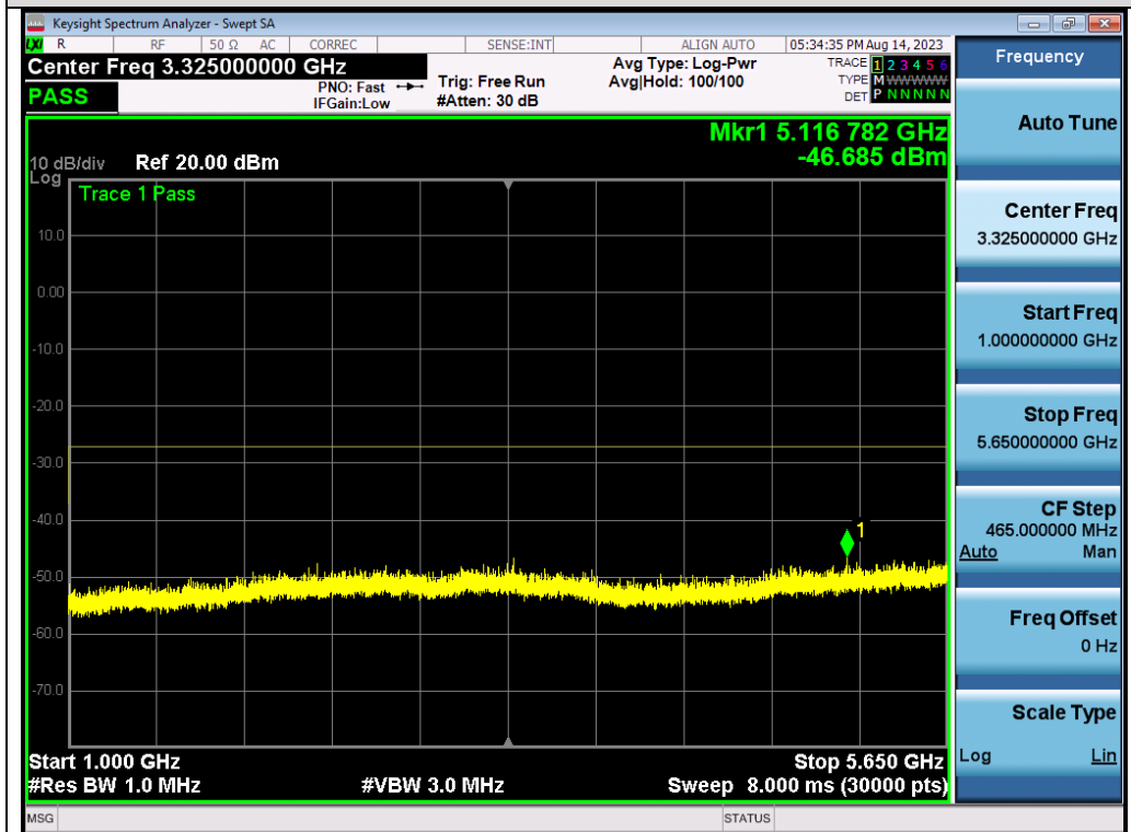
Test_Graph_802.11n40_ANT1_5755_MCS0_Frequency Band2
